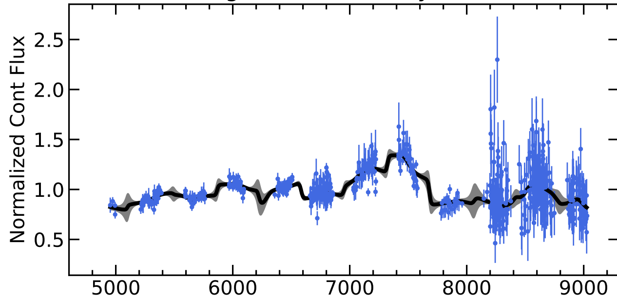
RM071 Light Curves (w/ PyROA model)
