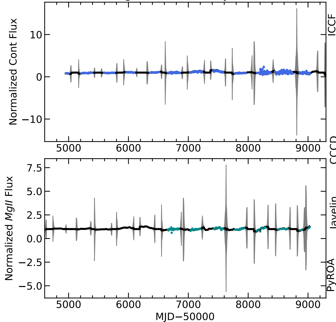
RM071 Light Curves (w/ PyROA model)
