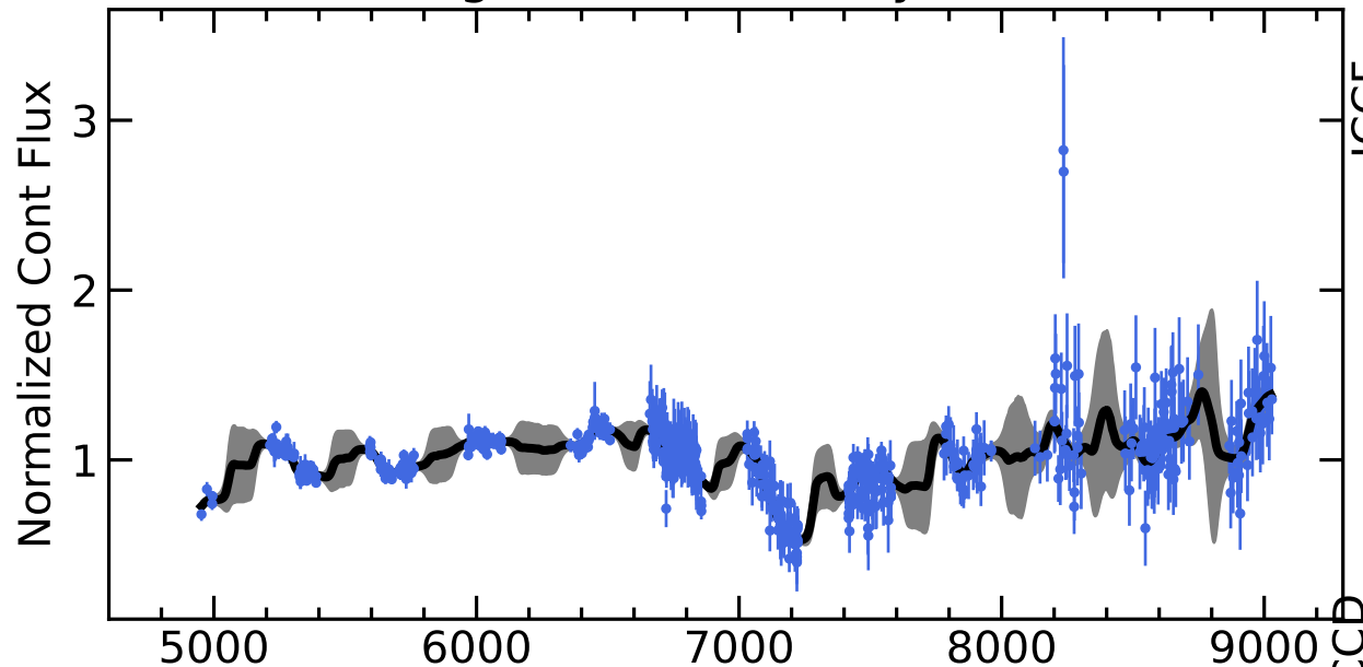
RM074 Light Curves (w/ PyROA model)
