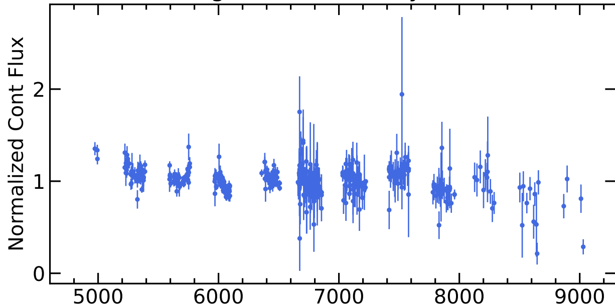
RM077 Light Curves (w/ PyROA model)
