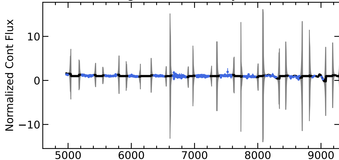
RM077 Light Curves (w/ PyROA model)
