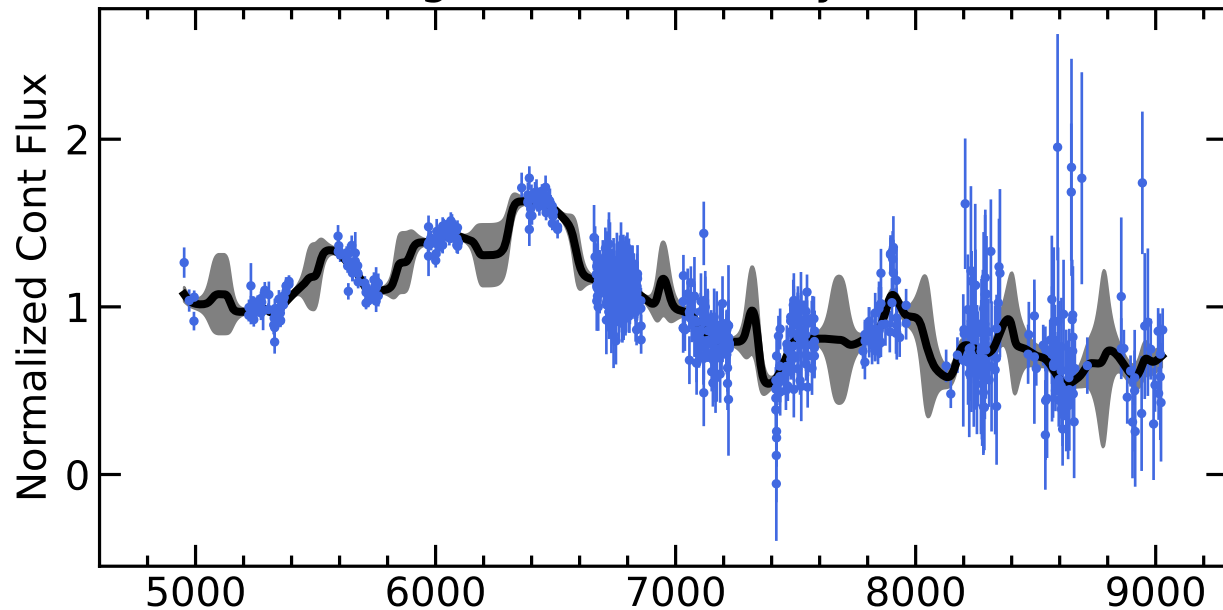
RM079 Light Curves (w/ PyROA model)
