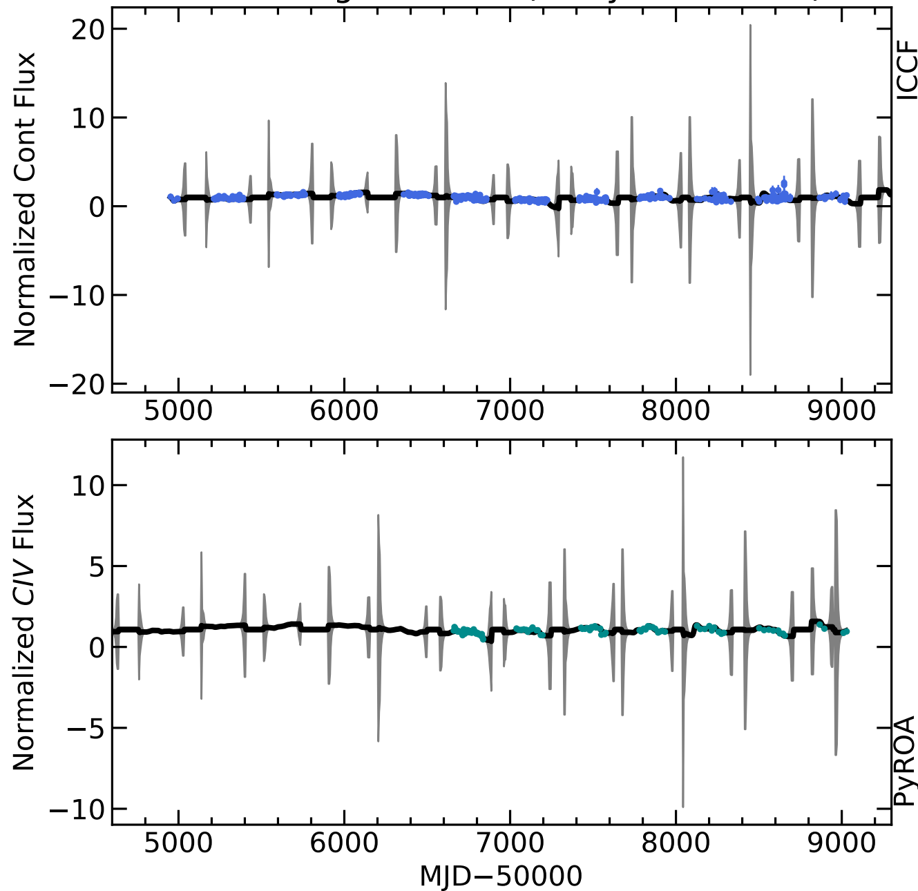
RM080 Light Curves (w/ PyROA model)
