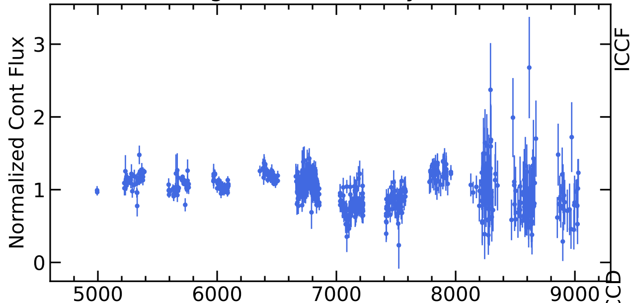
RM082 Light Curves (w/ PyROA model)
