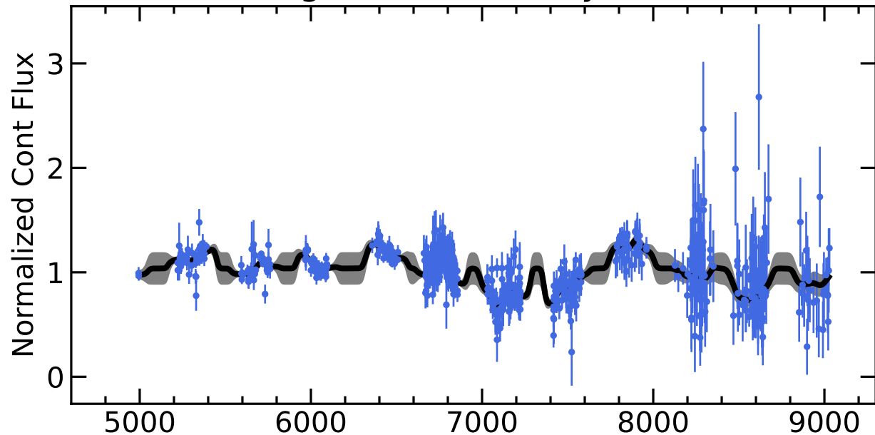
RM082 Light Curves (w/ PyROA model)
