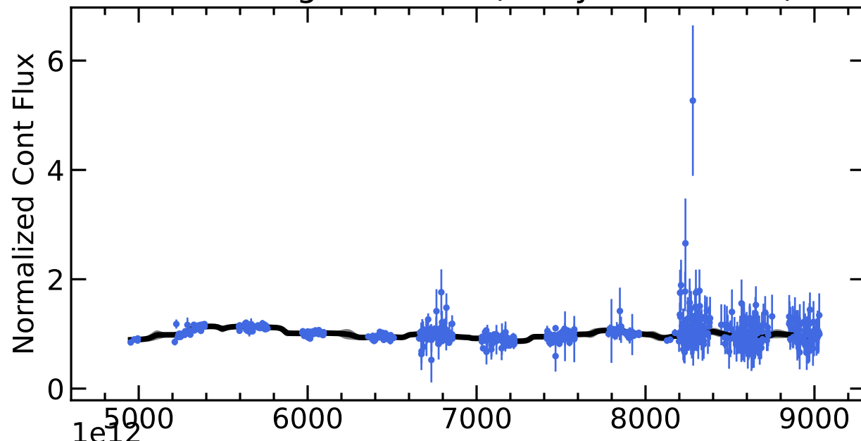
RM084 Light Curves (w/ PyROA model)
