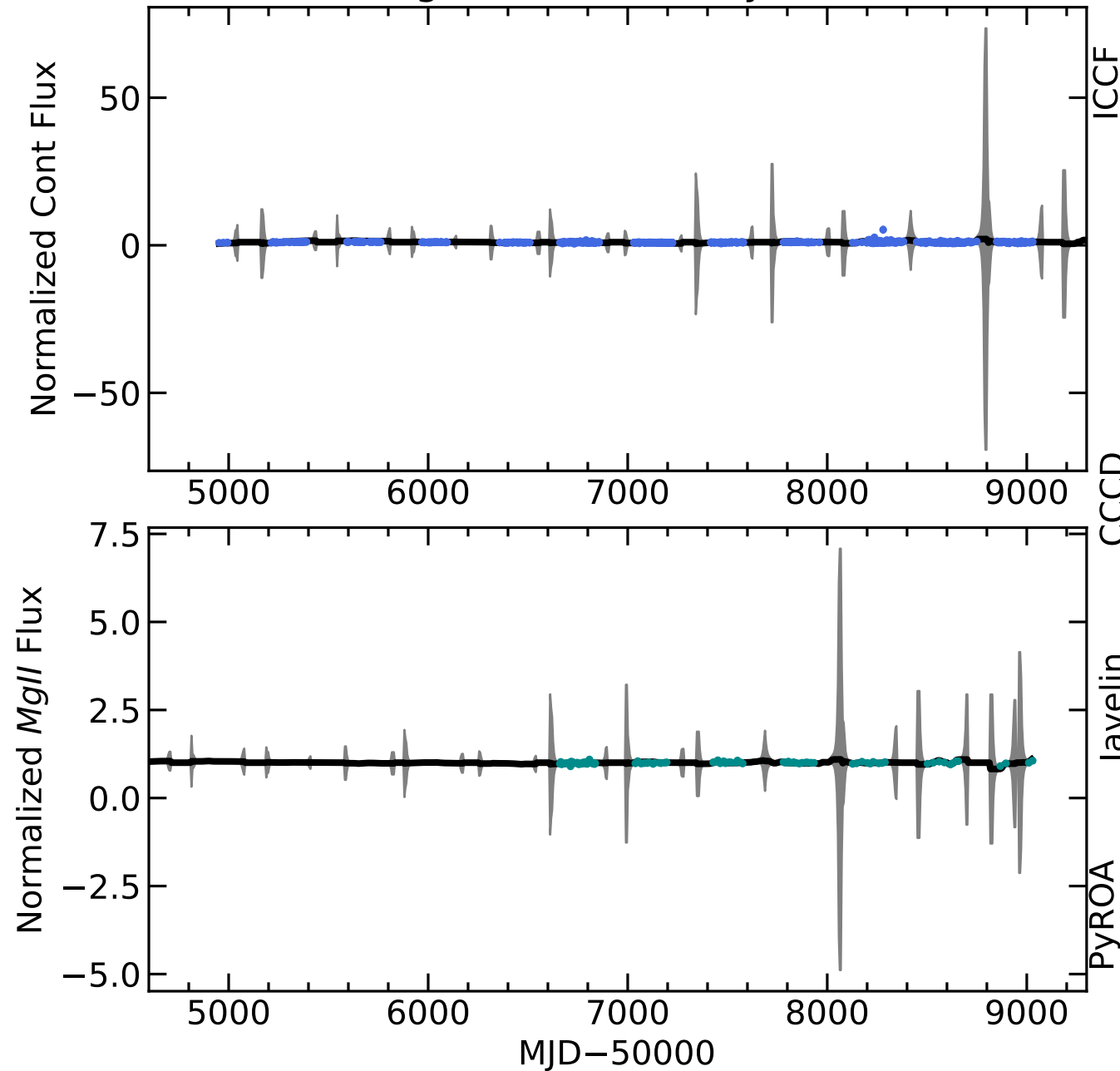
RM084 Light Curves (w/ PyROA model)
