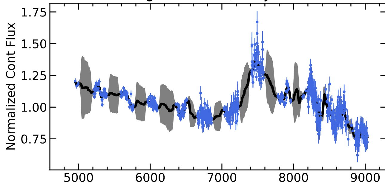
RM085 Light Curves (w/ PyROA model)
