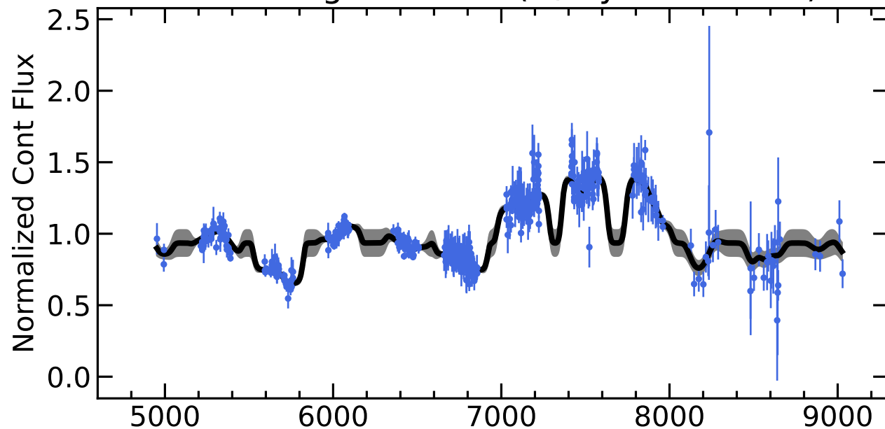
RM086 Light Curves (w/ PyROA model)
