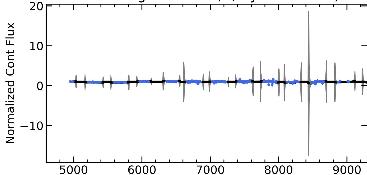
RM087 Light Curves (w/ PyROA model)
