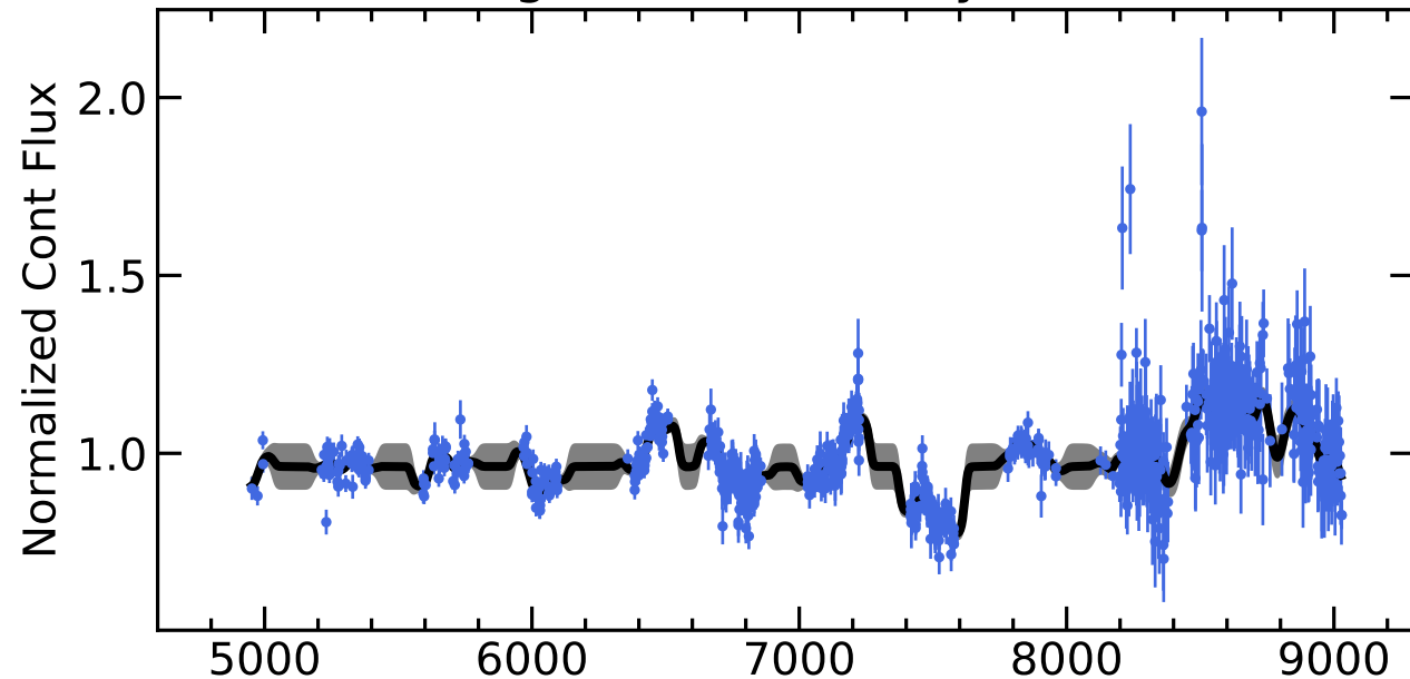
RM088 Light Curves (w/ PyROA model)
