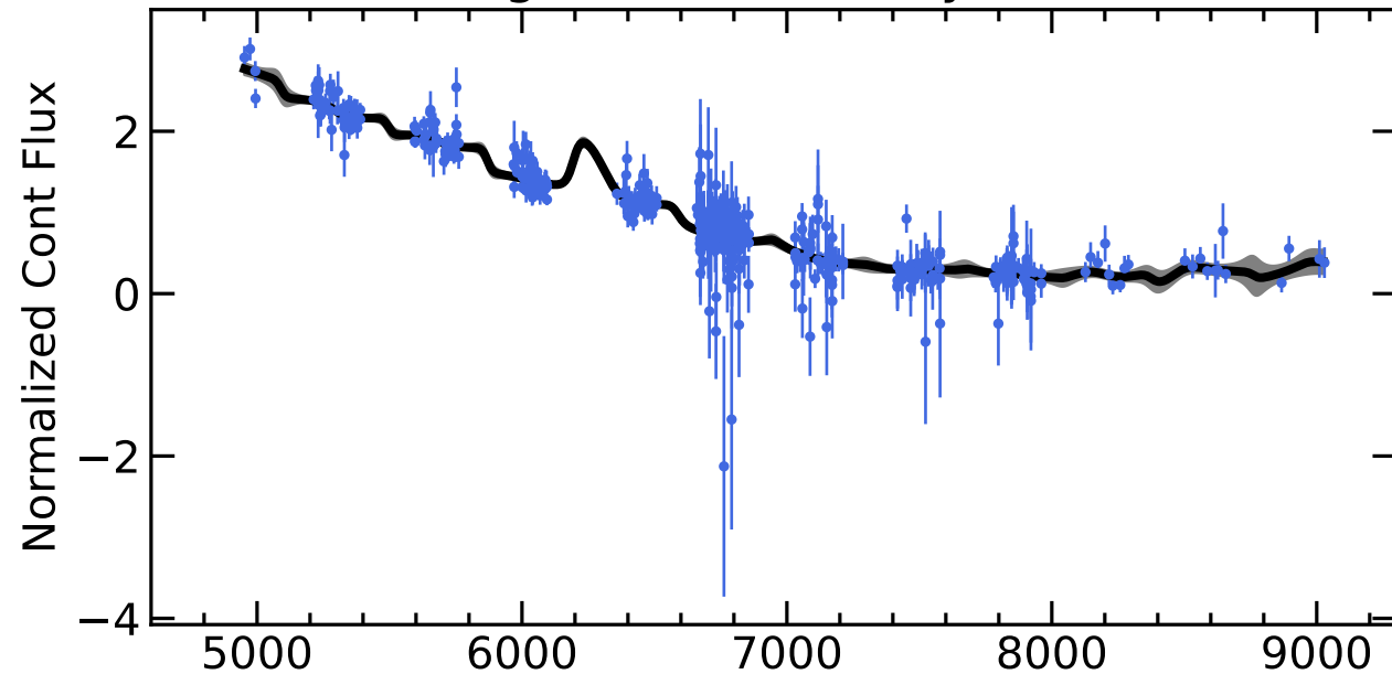
RM090 Light Curves (w/ PyROA model)
