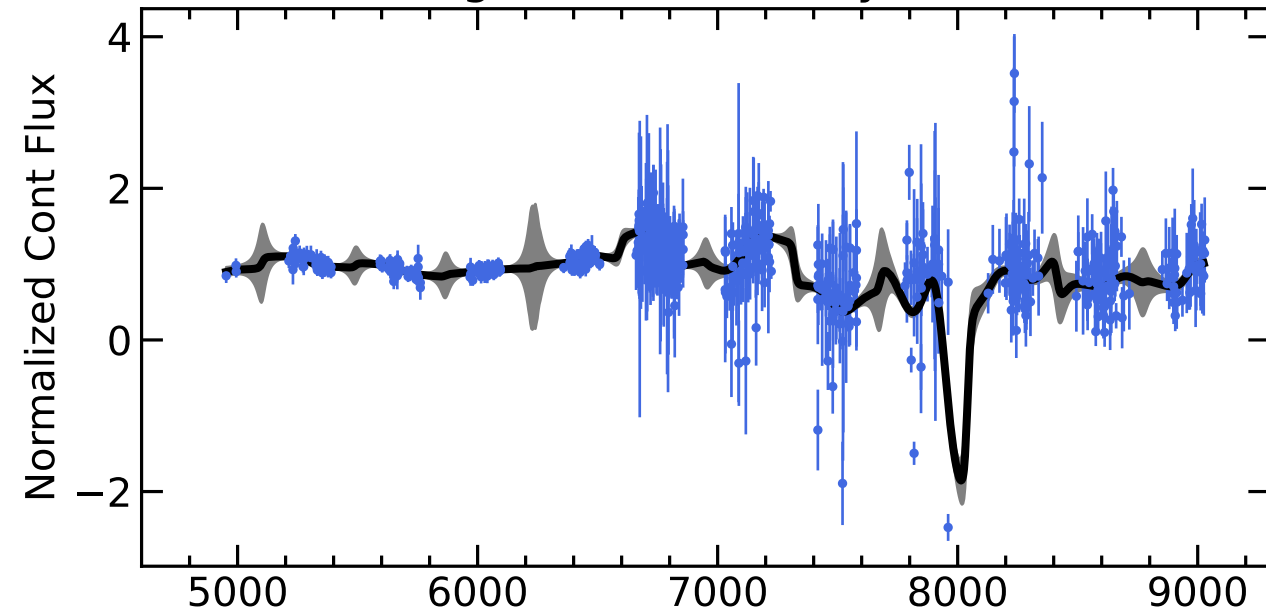
RM091 Light Curves (w/ PyROA model)
