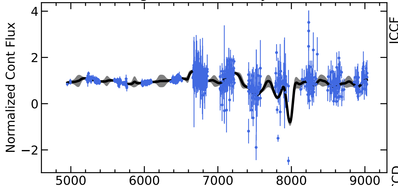
RM091 Light Curves (w/ PyROA model)
