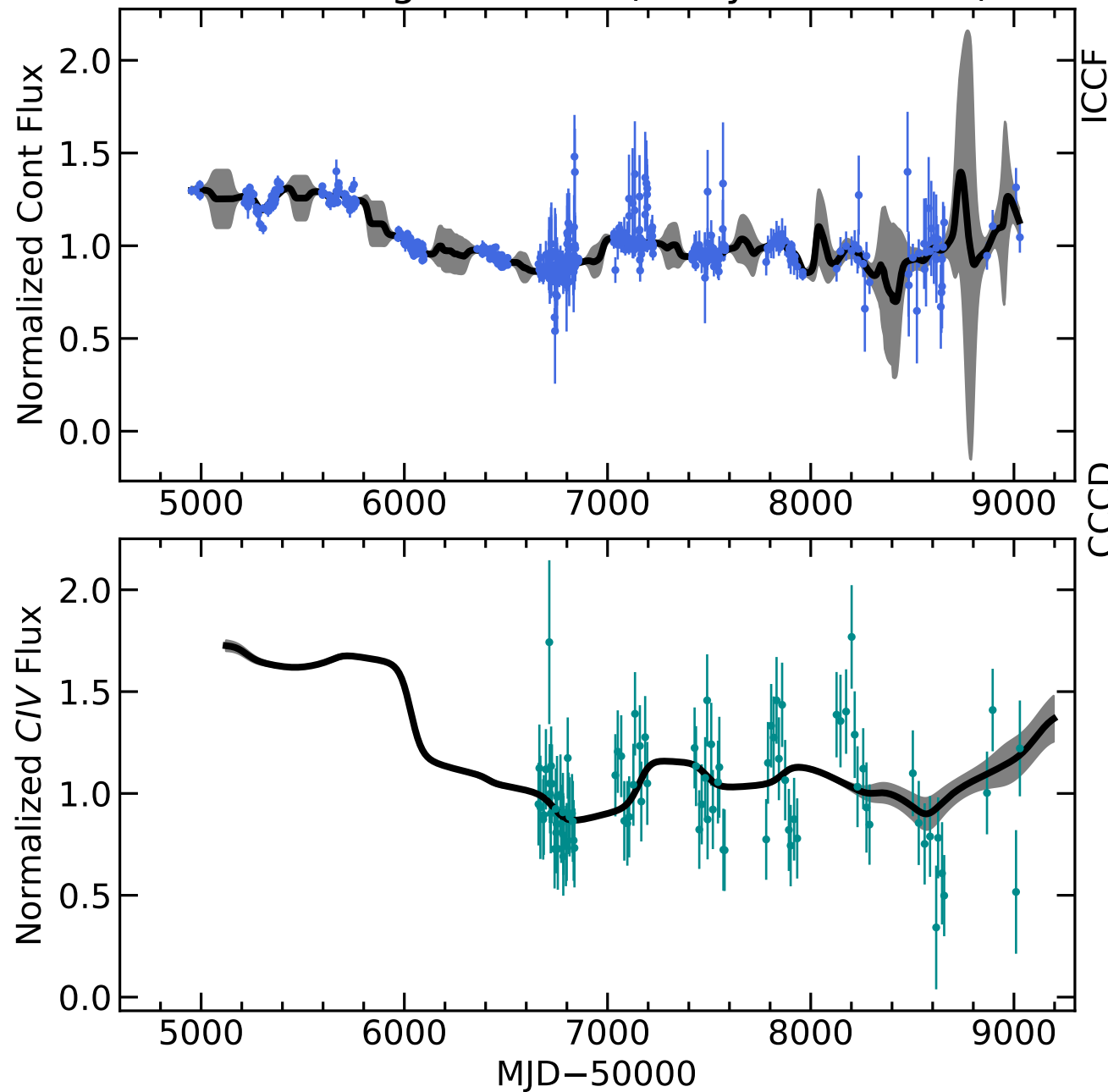
RM092 Light Curves (w/ PyROA model)
