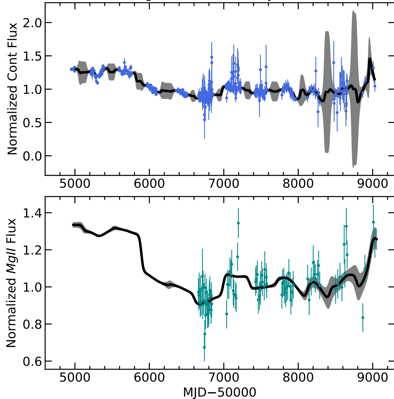
RM092 Light Curves (w/ PyROA model)
