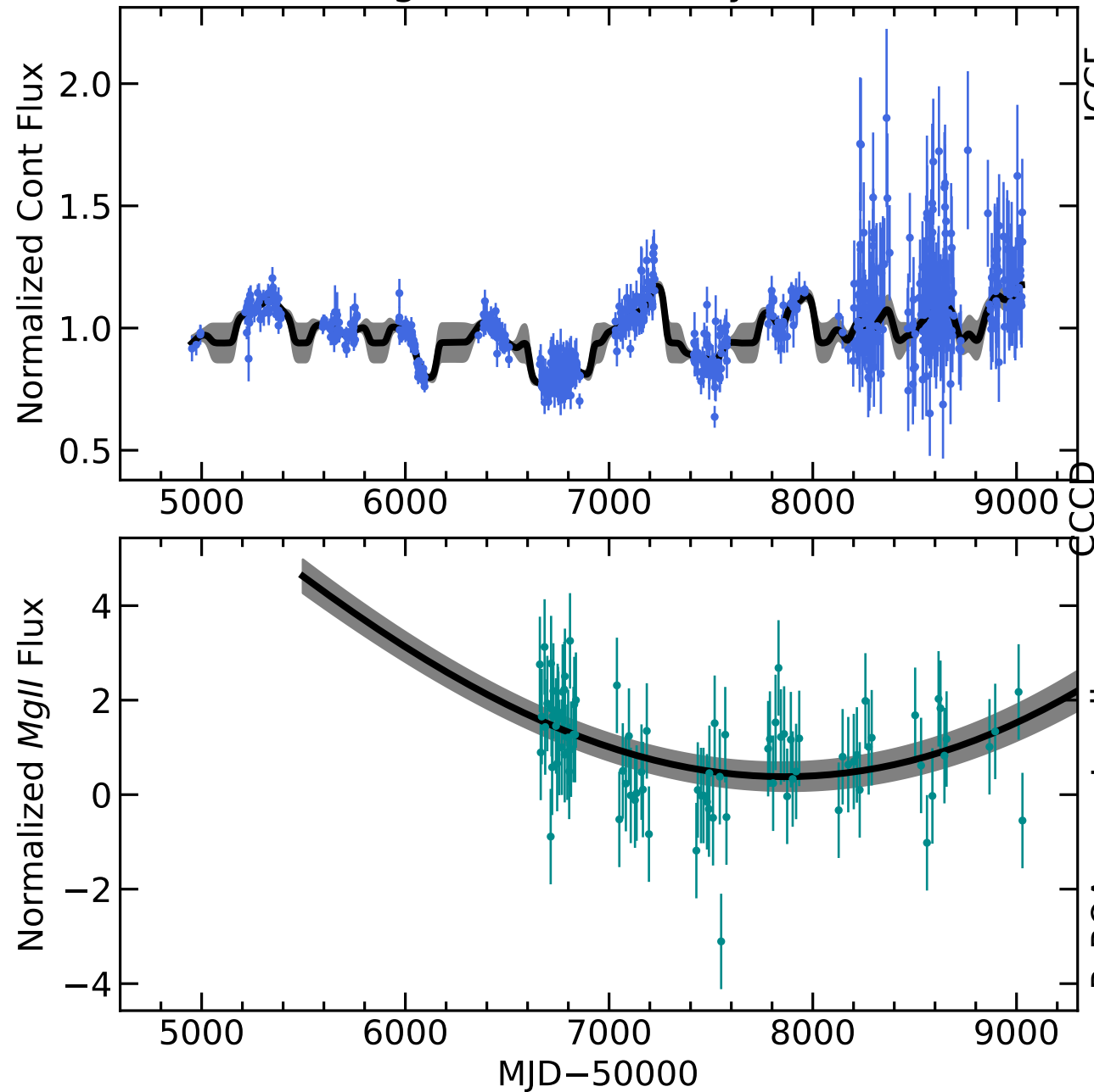
RM093 Light Curves (w/ PyROA model)
