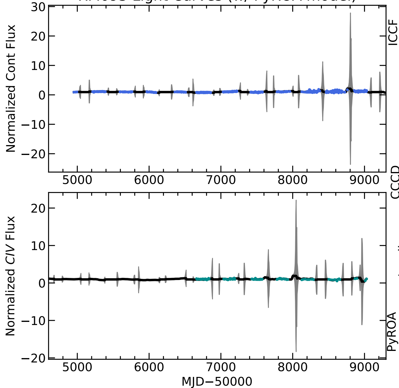
RM093 Light Curves (w/ PyROA model)
