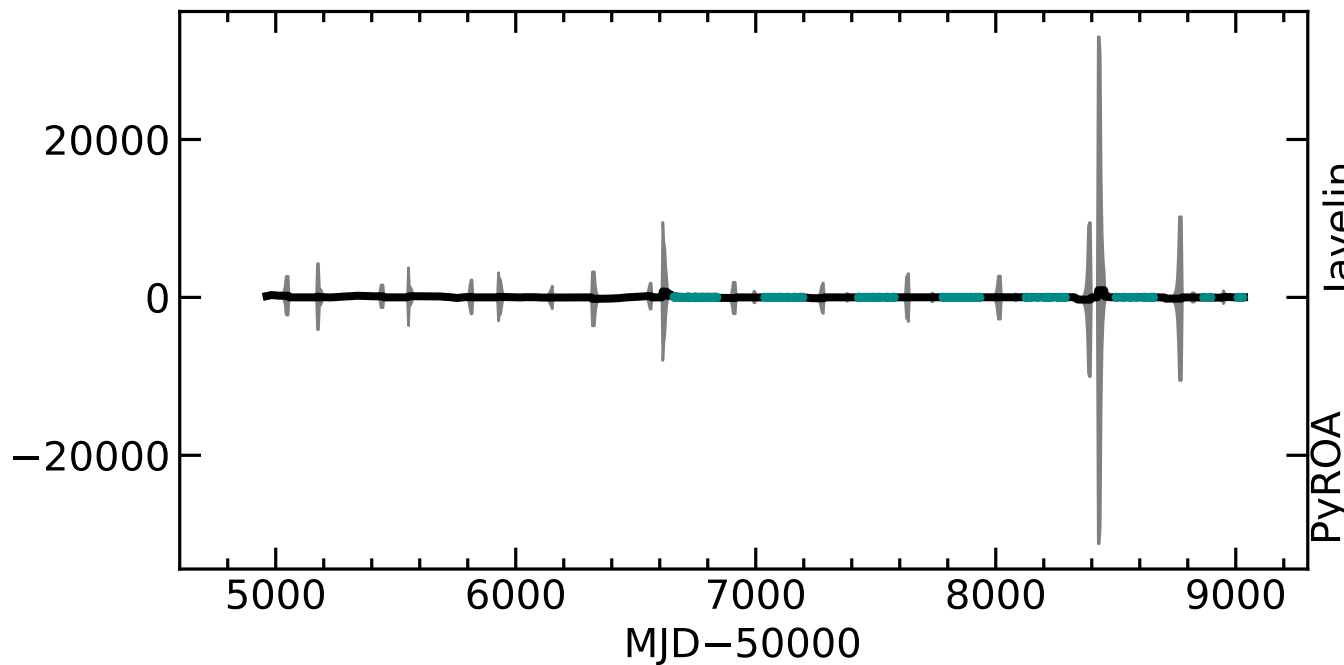
Normalized H\beta Flux
