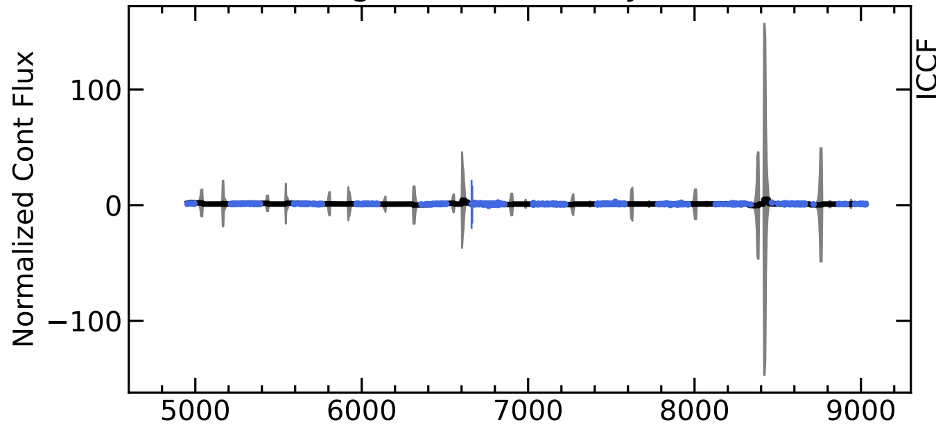
RM094 Light Curves (w/ PyROA model)
