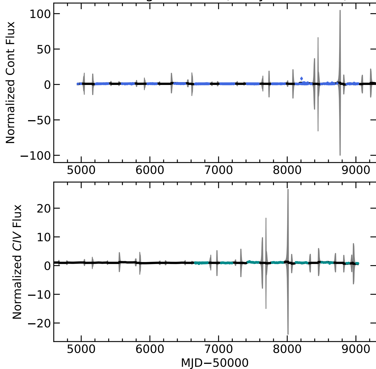
RM095 Light Curves (w/ PyROA model)
