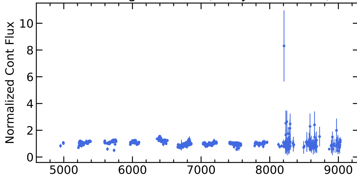
RM095 Light Curves (w/ PyROA model)
