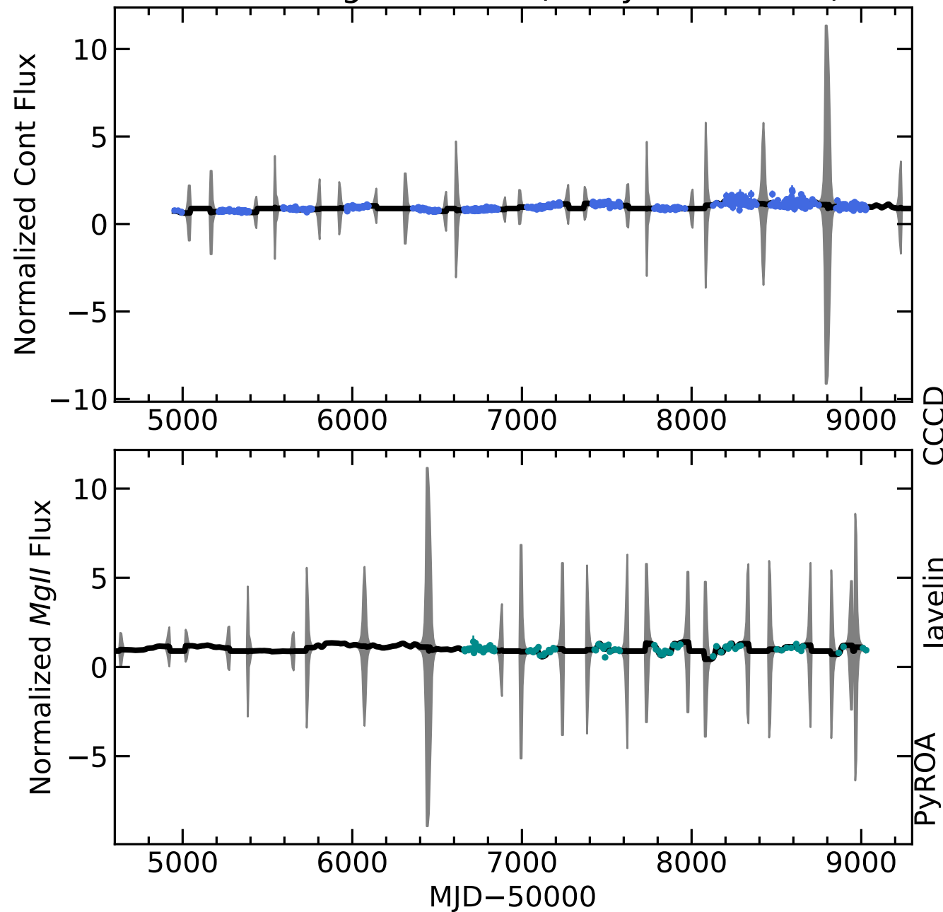
RM096 Light Curves (w/ PyROA model)
