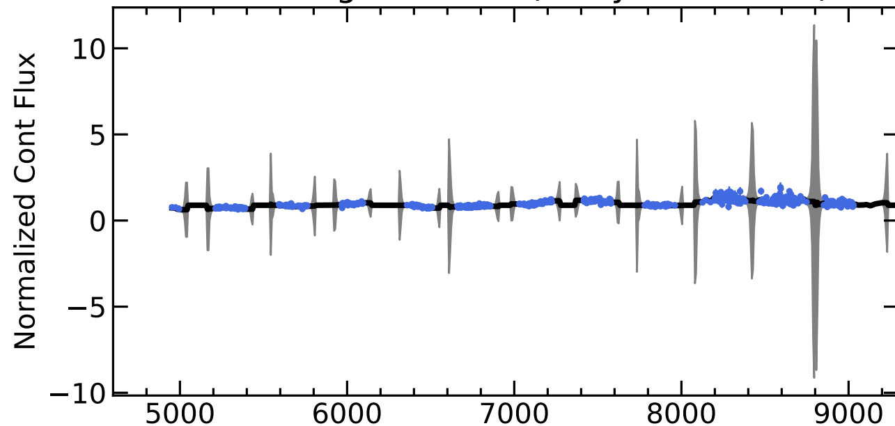
RM096 Light Curves (w/ PyROA model)
