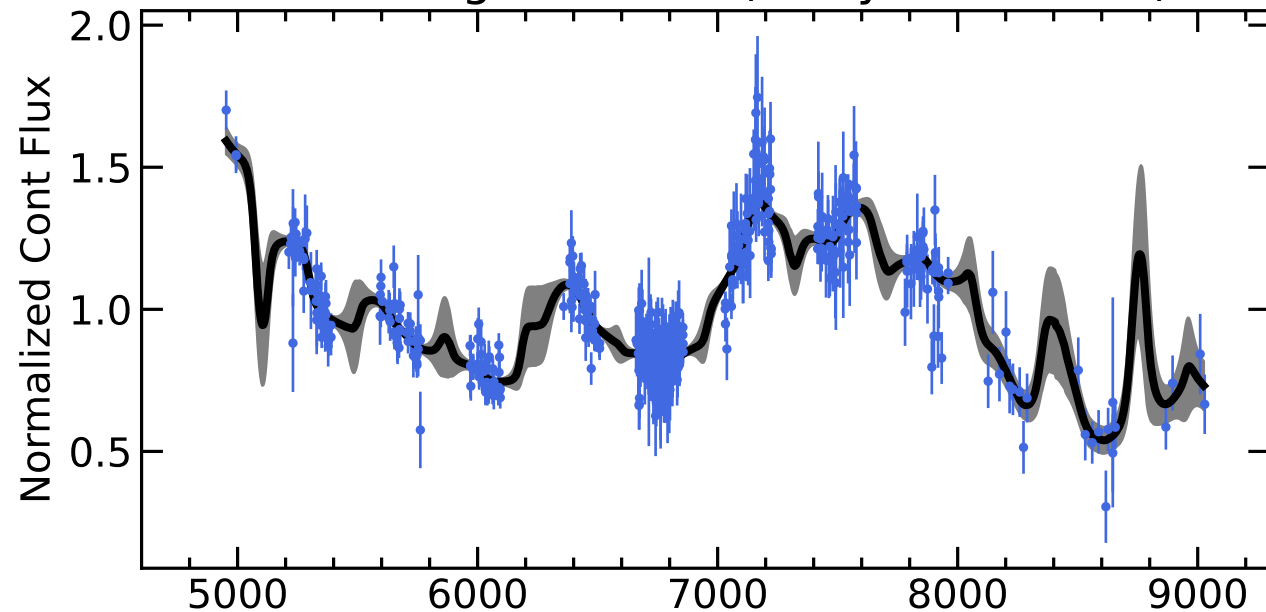
RM097 Light Curves (w/ PyROA model)
