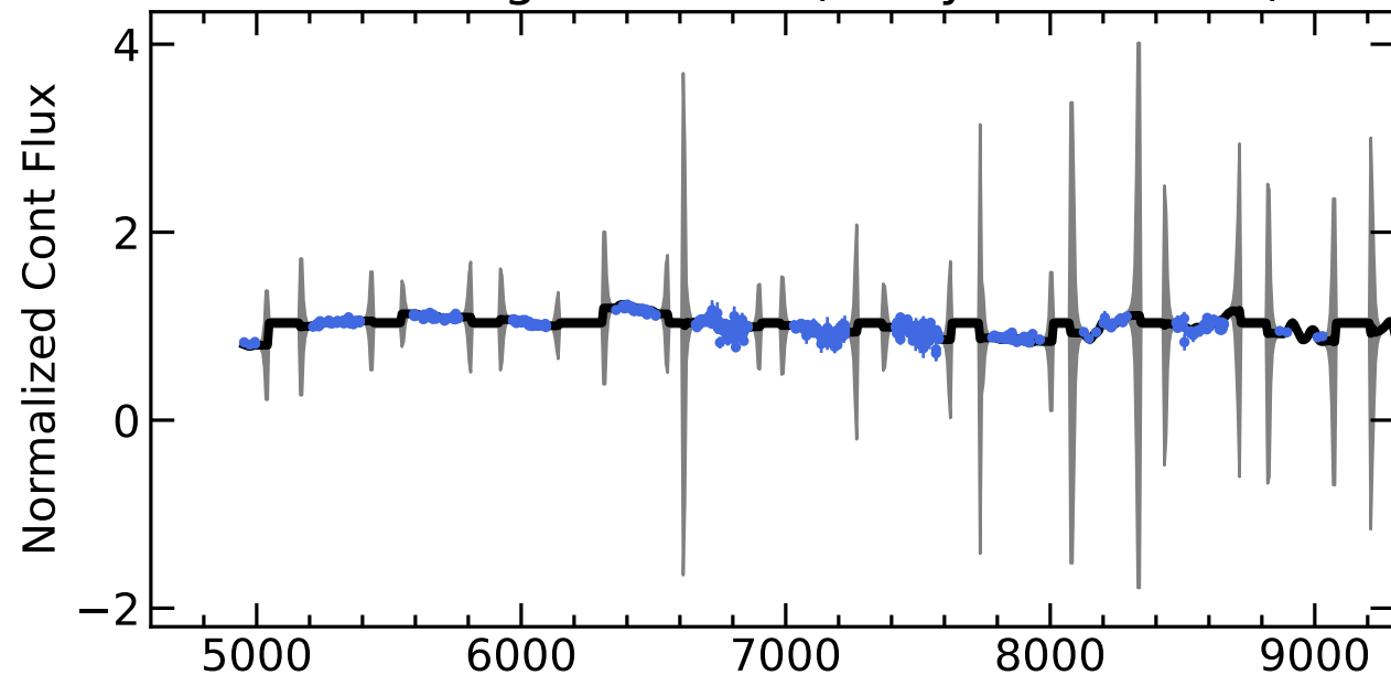
RM100 Light Curves (w/ PyROA model)
