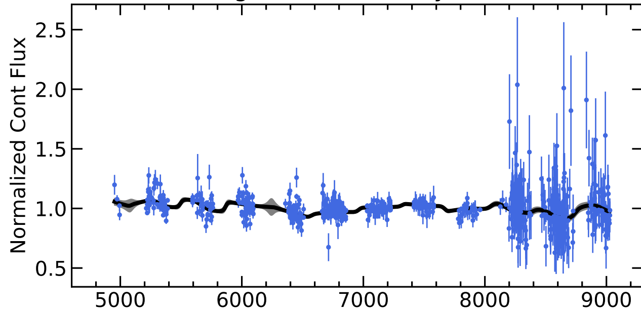
RM103 Light Curves (w/ PyROA model)
