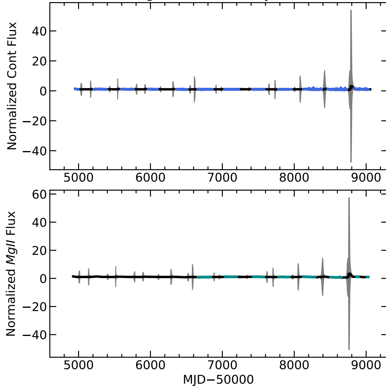
RM103 Light Curves (w/ PyROA model)
