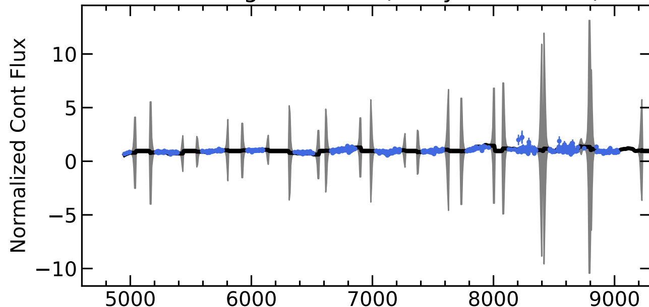
RM104 Light Curves (w/ PyROA model)
