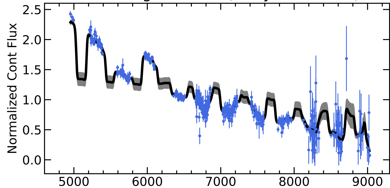
RM105 Light Curves (w/ PyROA model)
