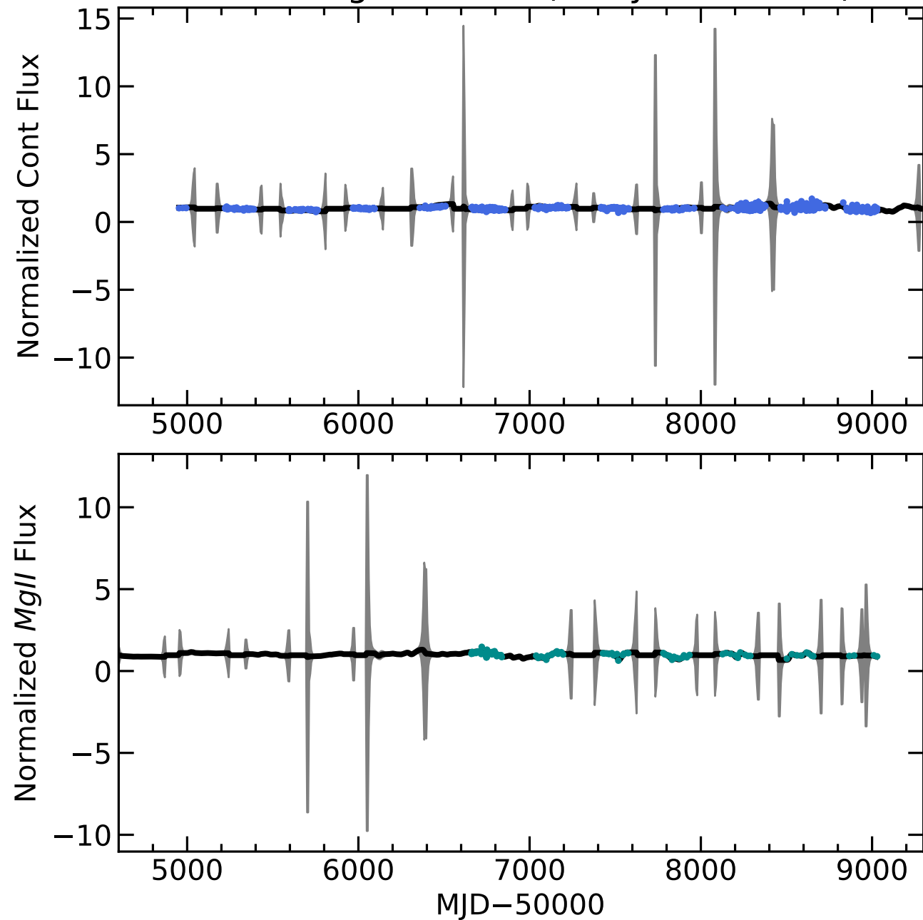
RM107 Light Curves (w/ PyROA model)
