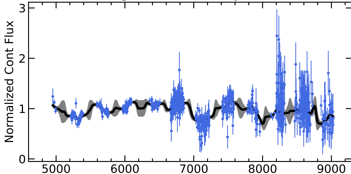
RM108 Light Curves (w/ PyROA model)
