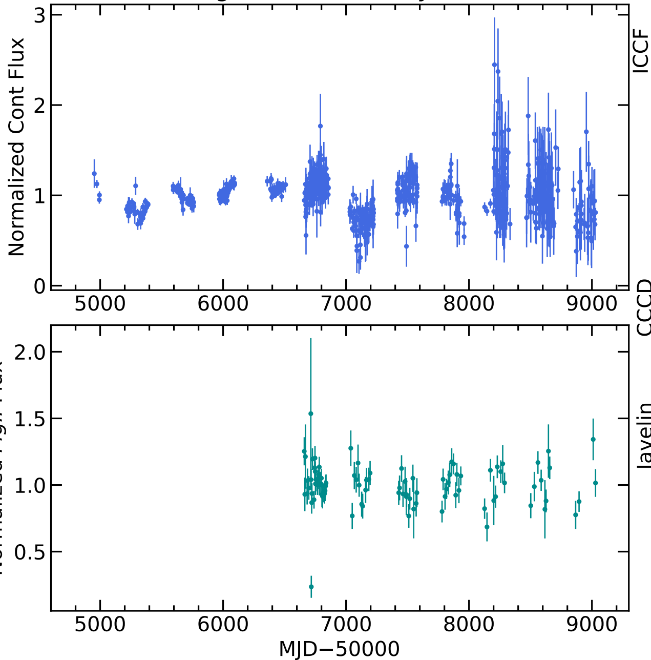
RM108 Light Curves (w/ PyROA model)
