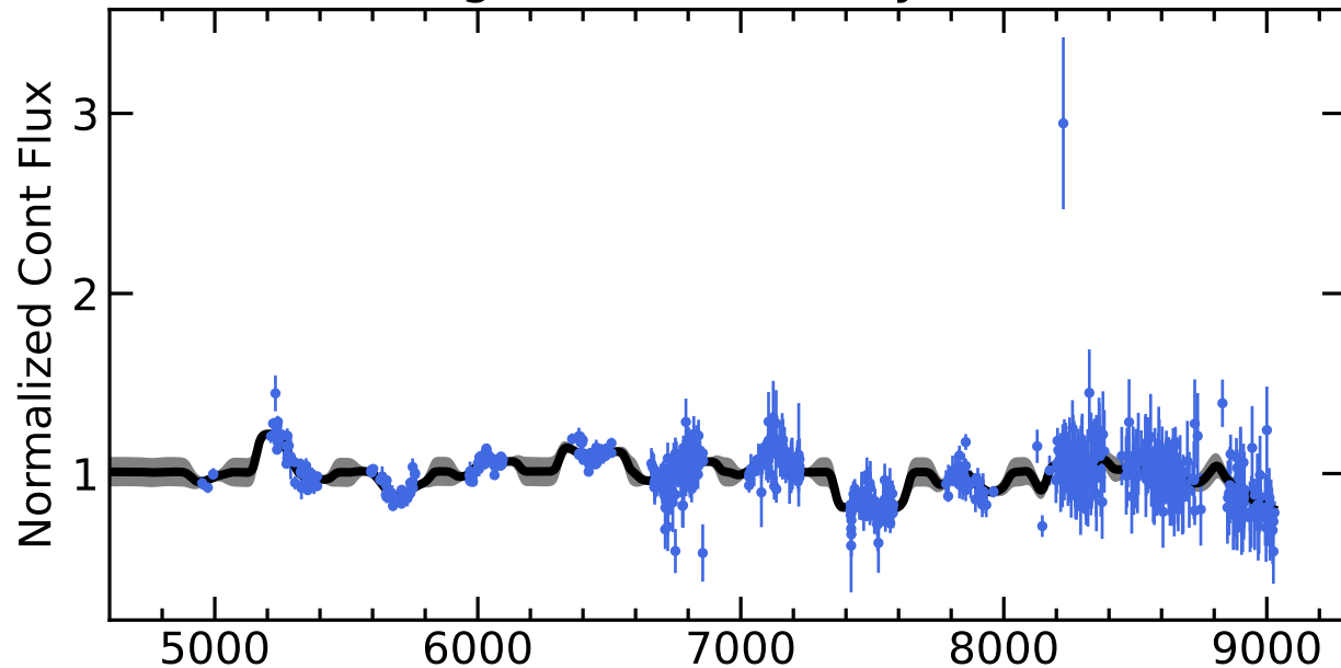
RM109 Light Curves (w/ PyROA model)
