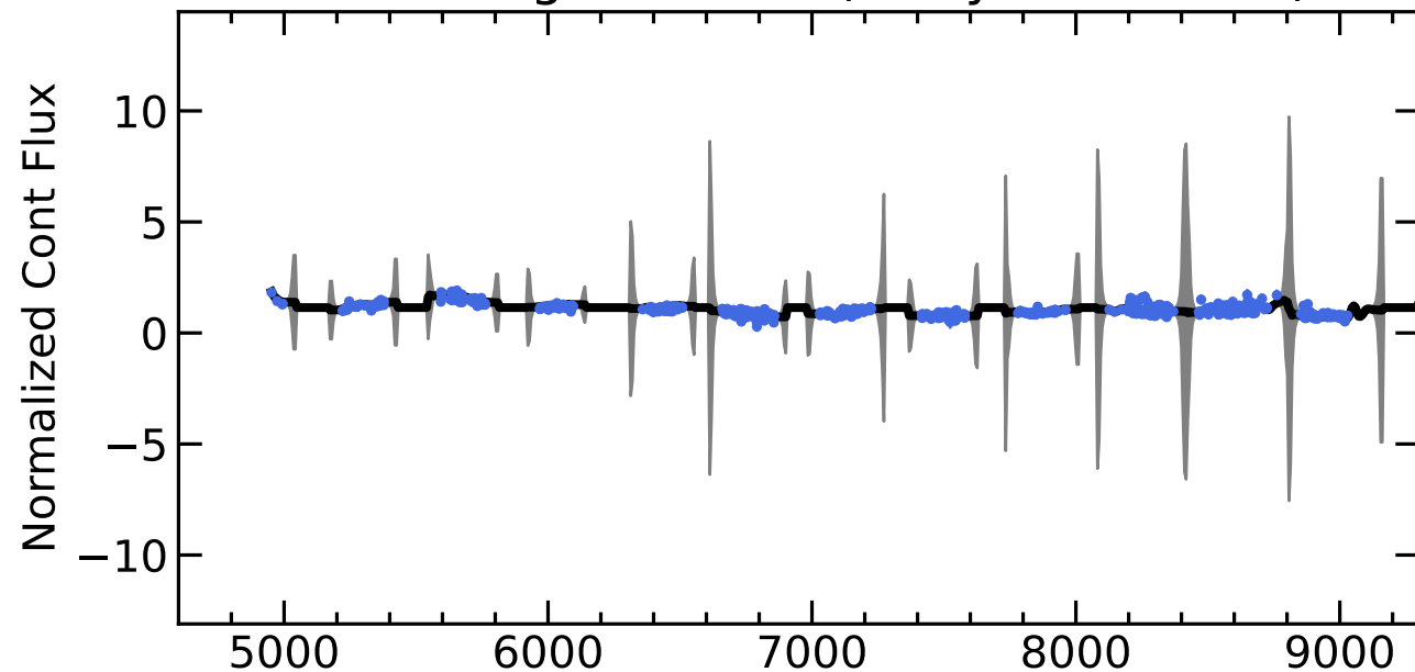
RM110 Light Curves (w/ PyROA model)
