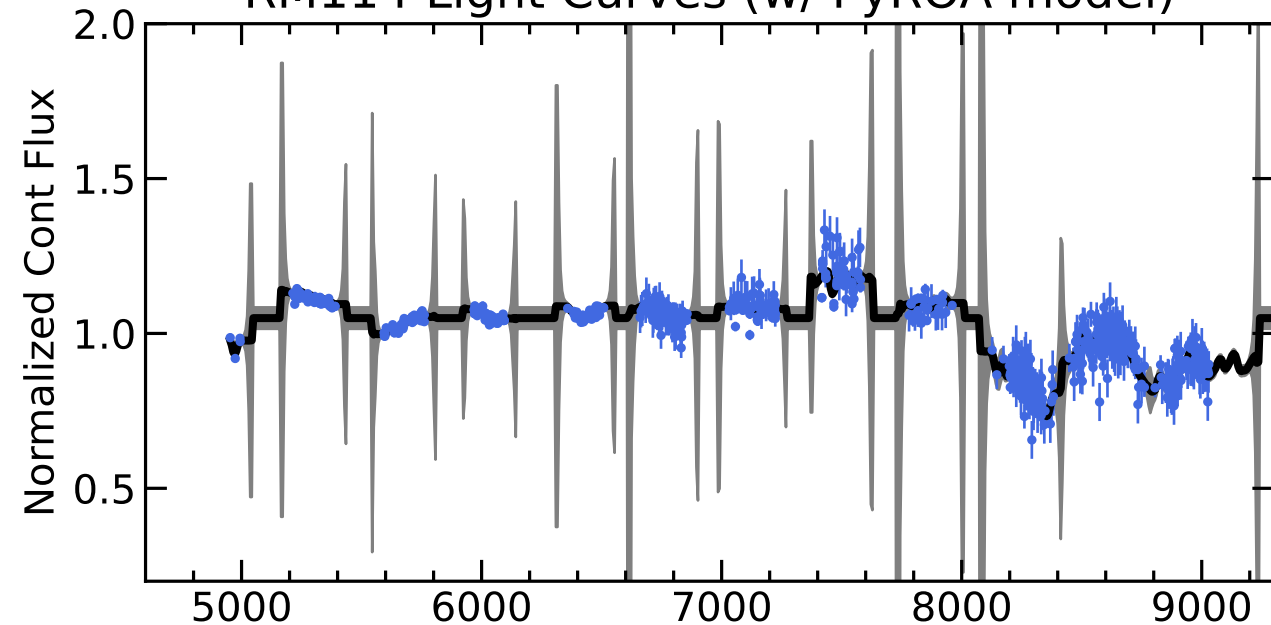
RM114 Light Curves (w/ PyROA model)
