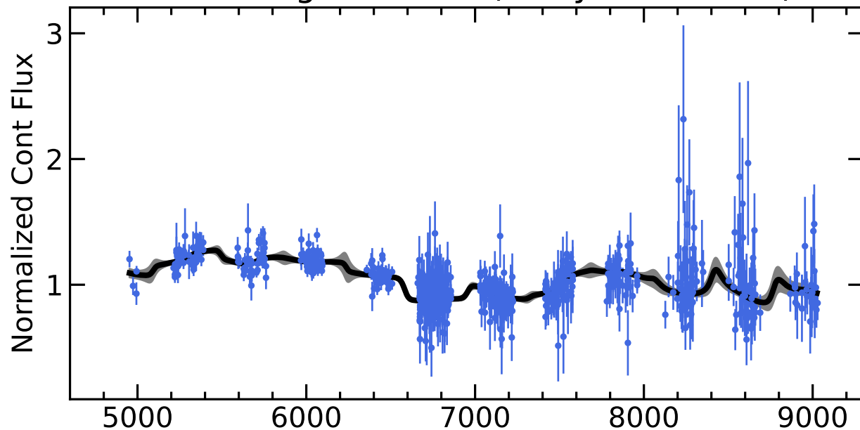
RM115 Light Curves (w/ PyROA model)
