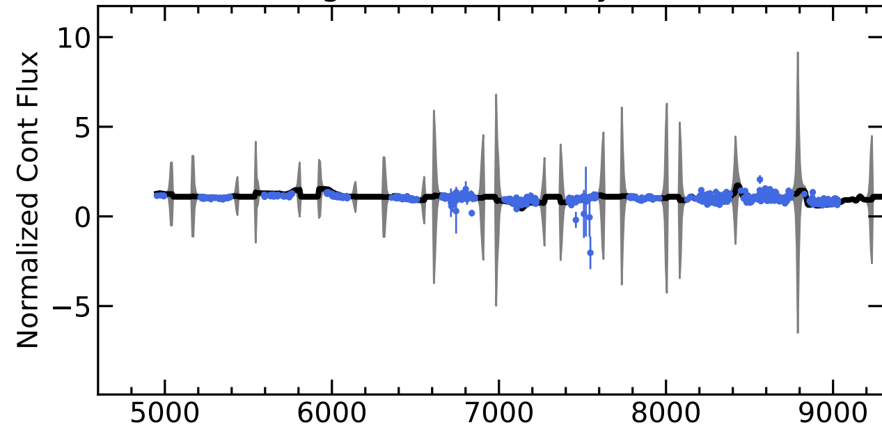
RM116 Light Curves (w/ PyROA model)
