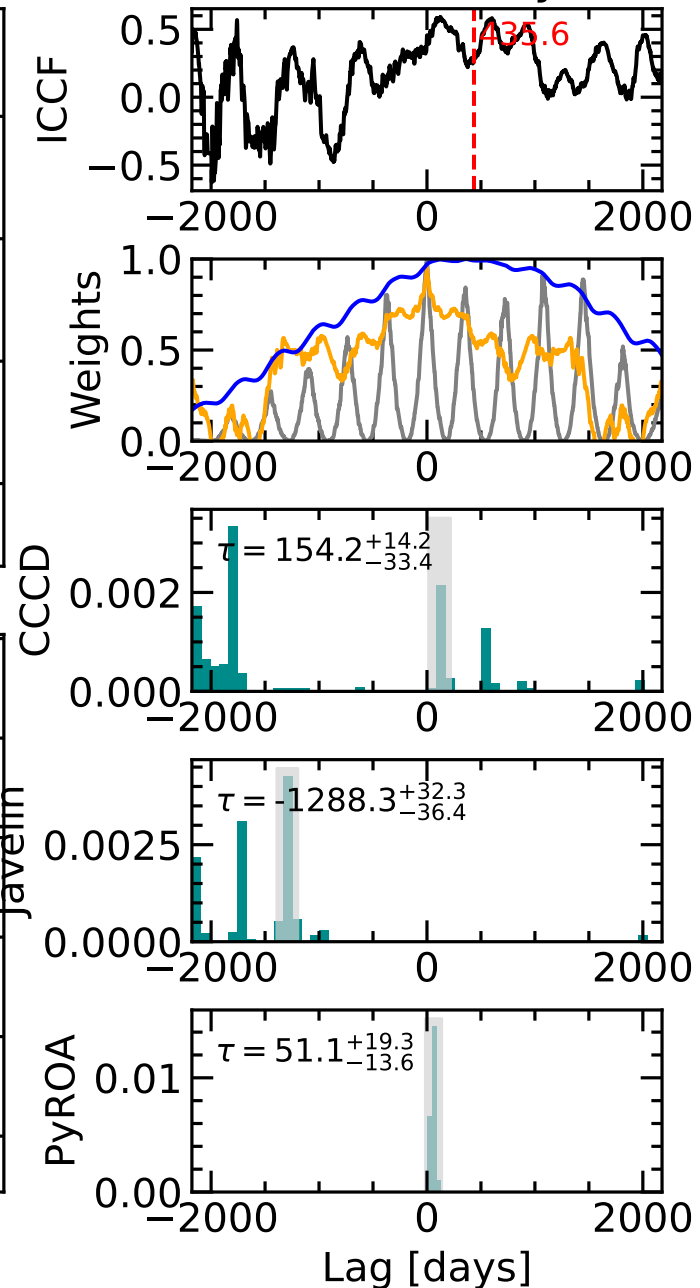
Time Delay
