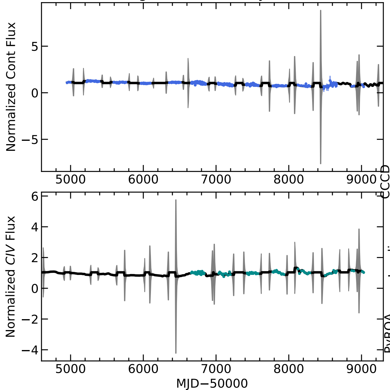
RM117 Light Curves (w/ PyROA model)
