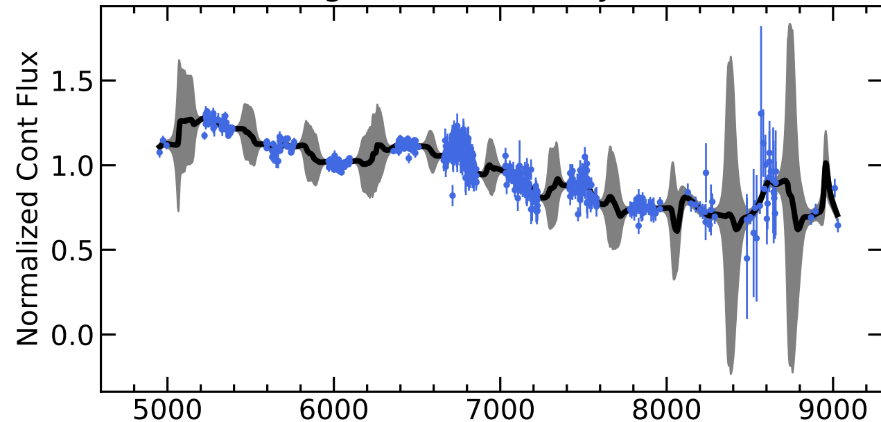
RM117 Light Curves (w/ PyROA model)
