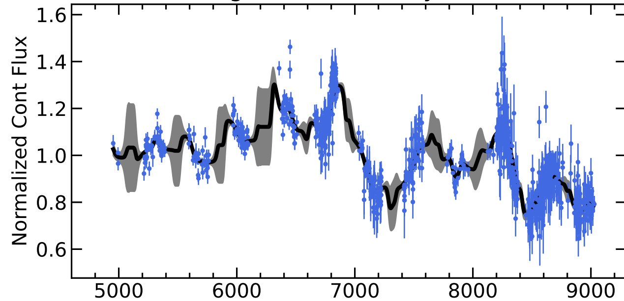
RM118 Light Curves (w/ PyROA model)
