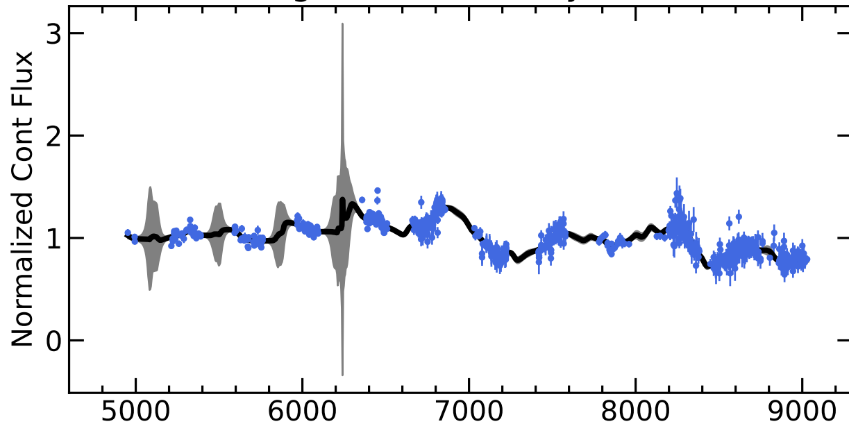
RM118 Light Curves (w/ PyROA model)
