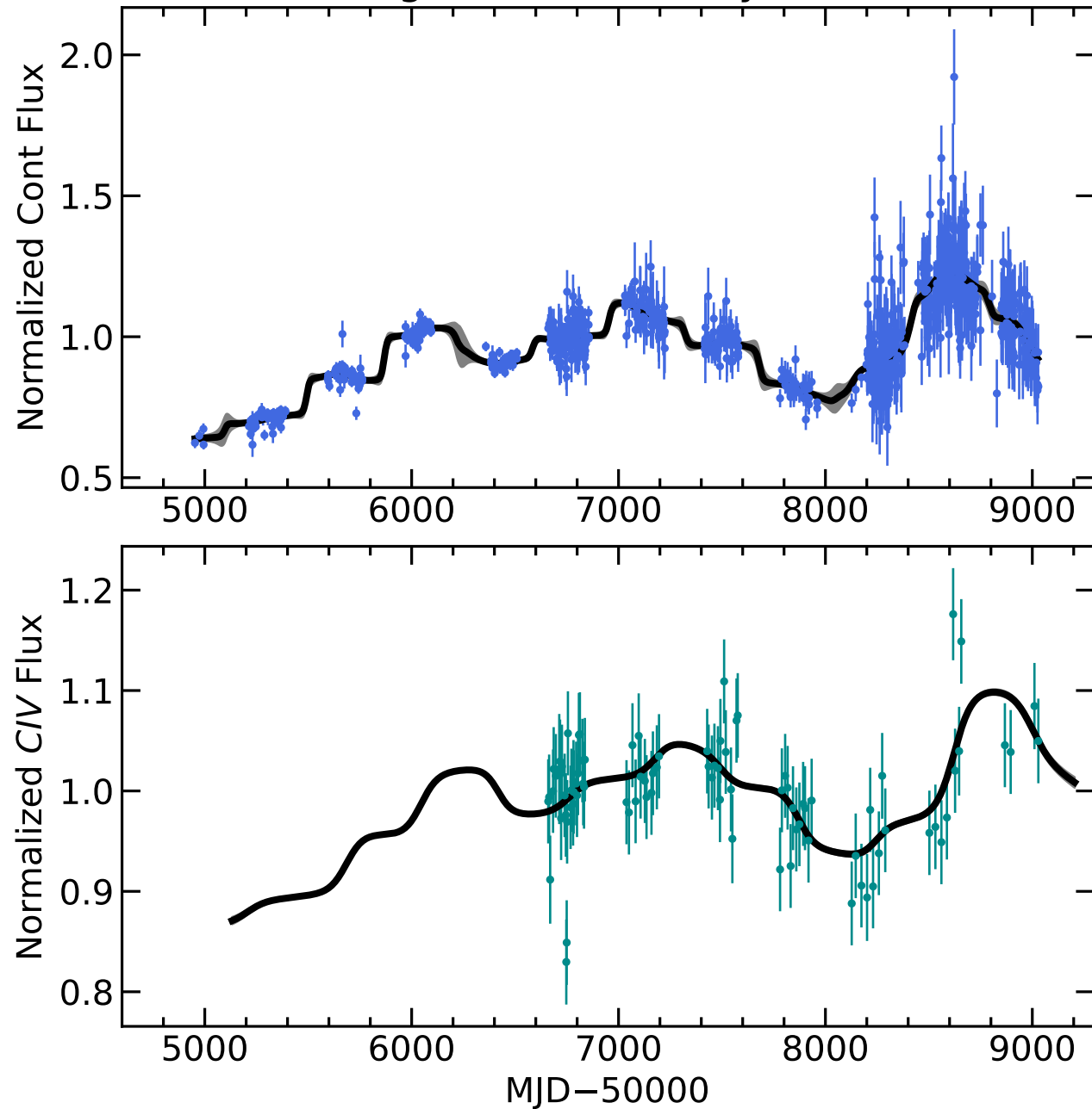
RM119 Light Curves (w/ PyROA model)
