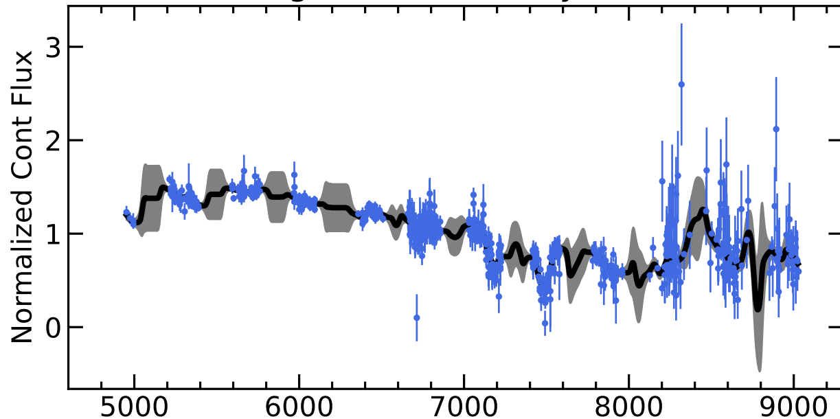
RM120 Light Curves (w/ PyROA model)
