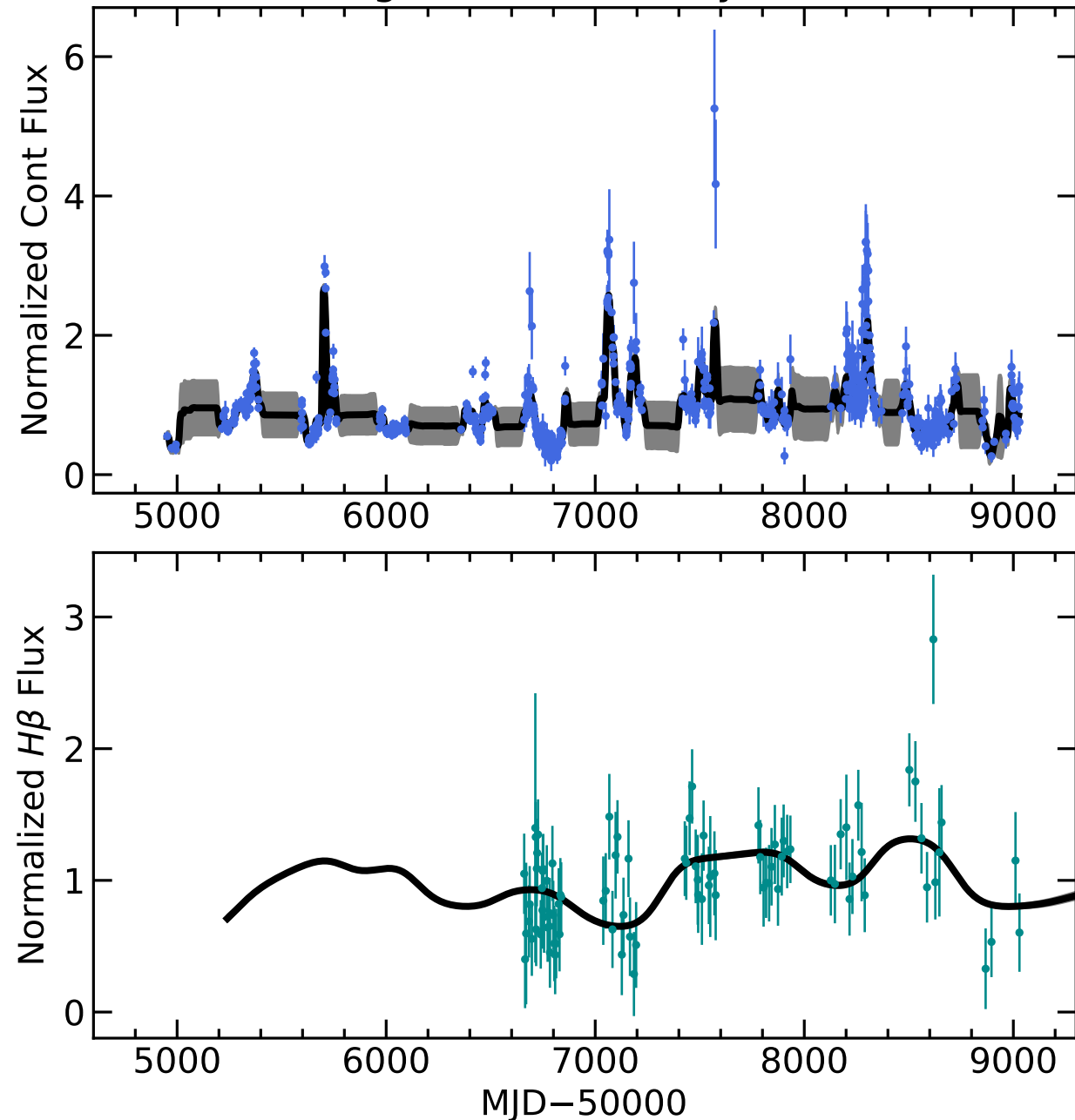
RM121 Light Curves (w/ PyROA model)
