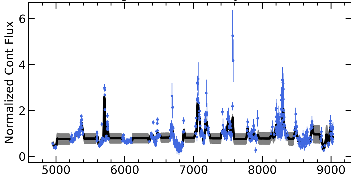
RM121 Light Curves (w/ PyROA model)
