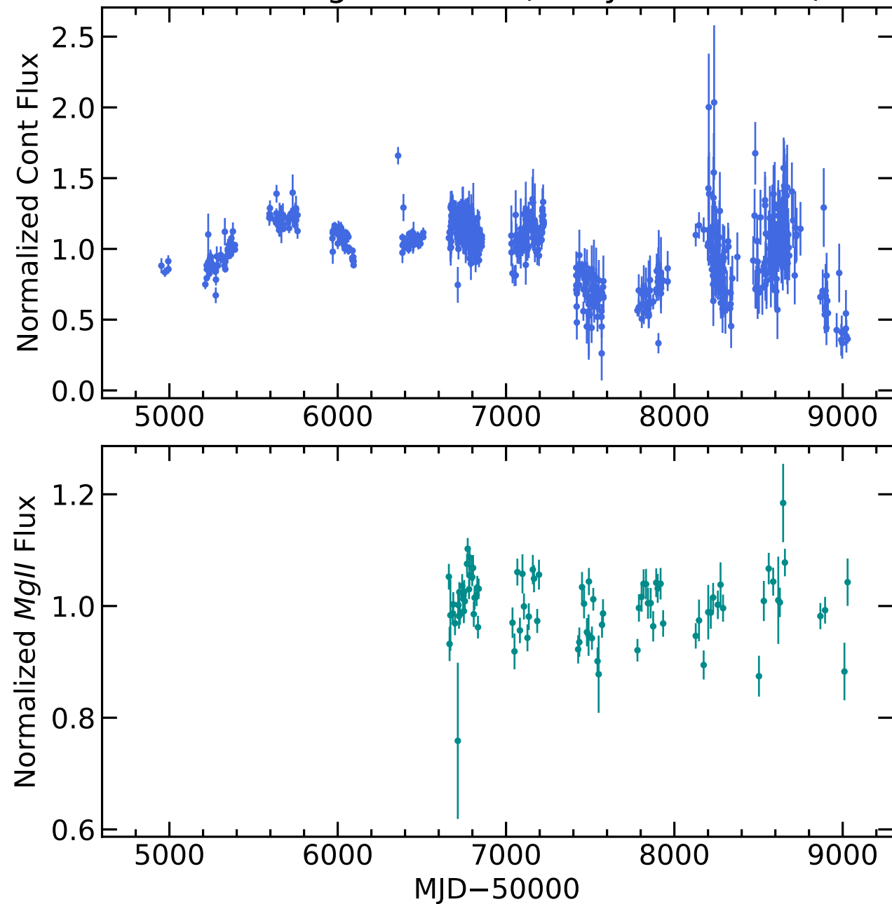
RM122 Light Curves (w/ PyROA model)
