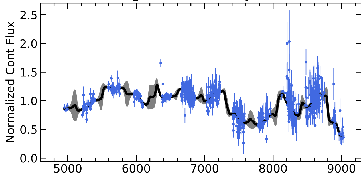
RM122 Light Curves (w/ PyROA model)
