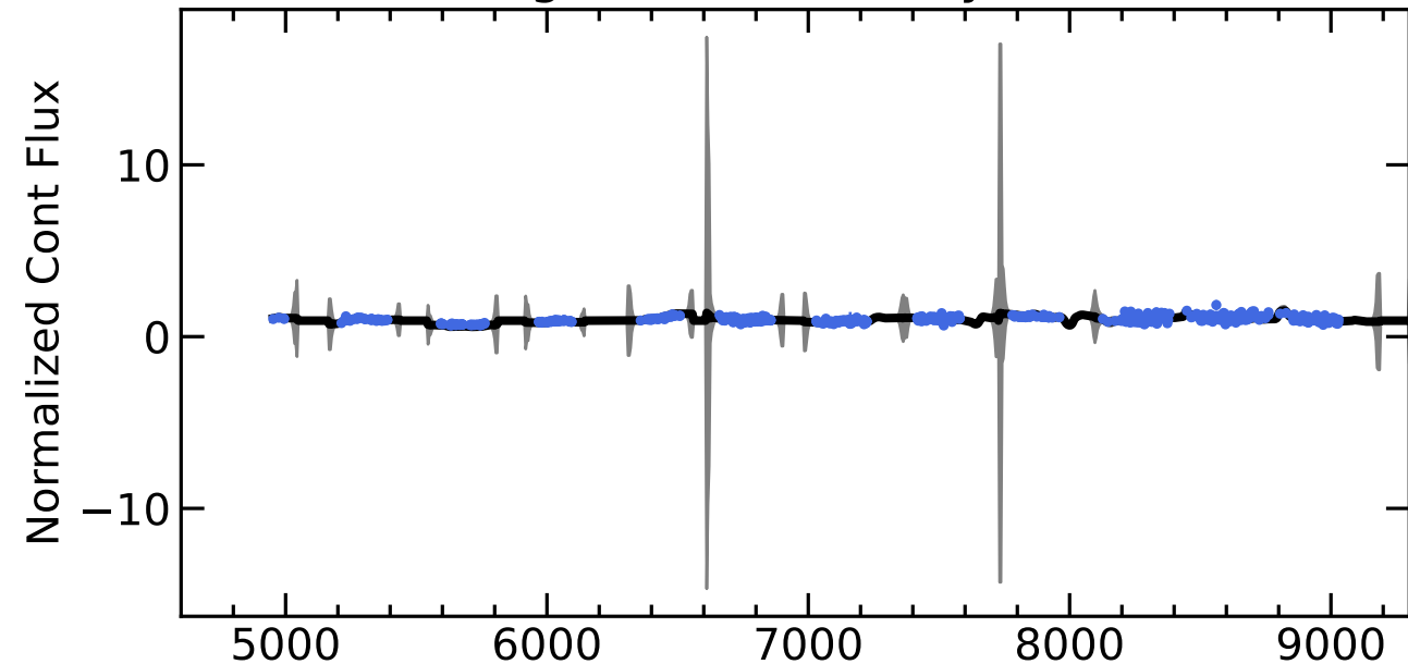
RM123 Light Curves (w/ PyROA model)
