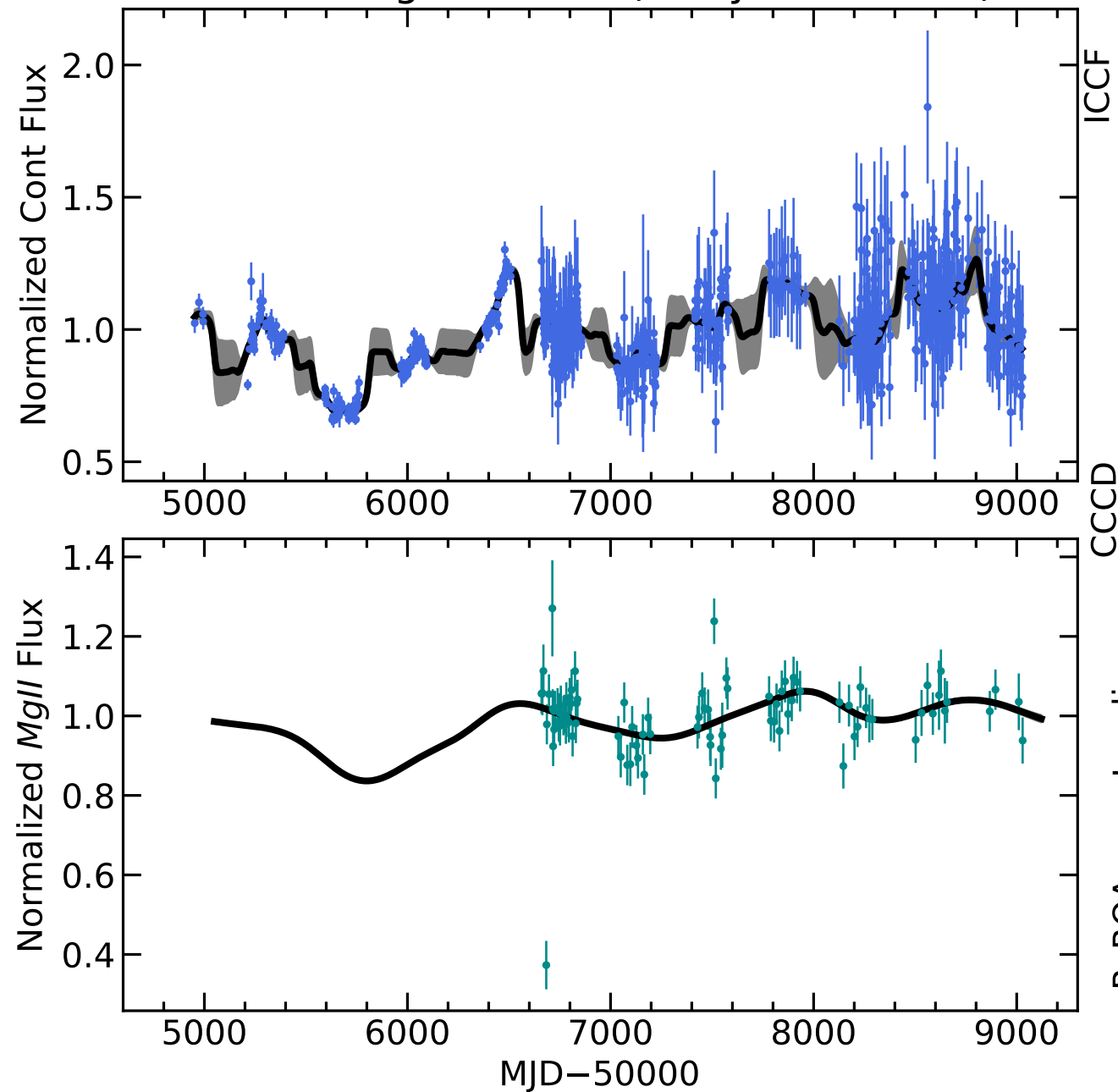
RM123 Light Curves (w/ PyROA model)
