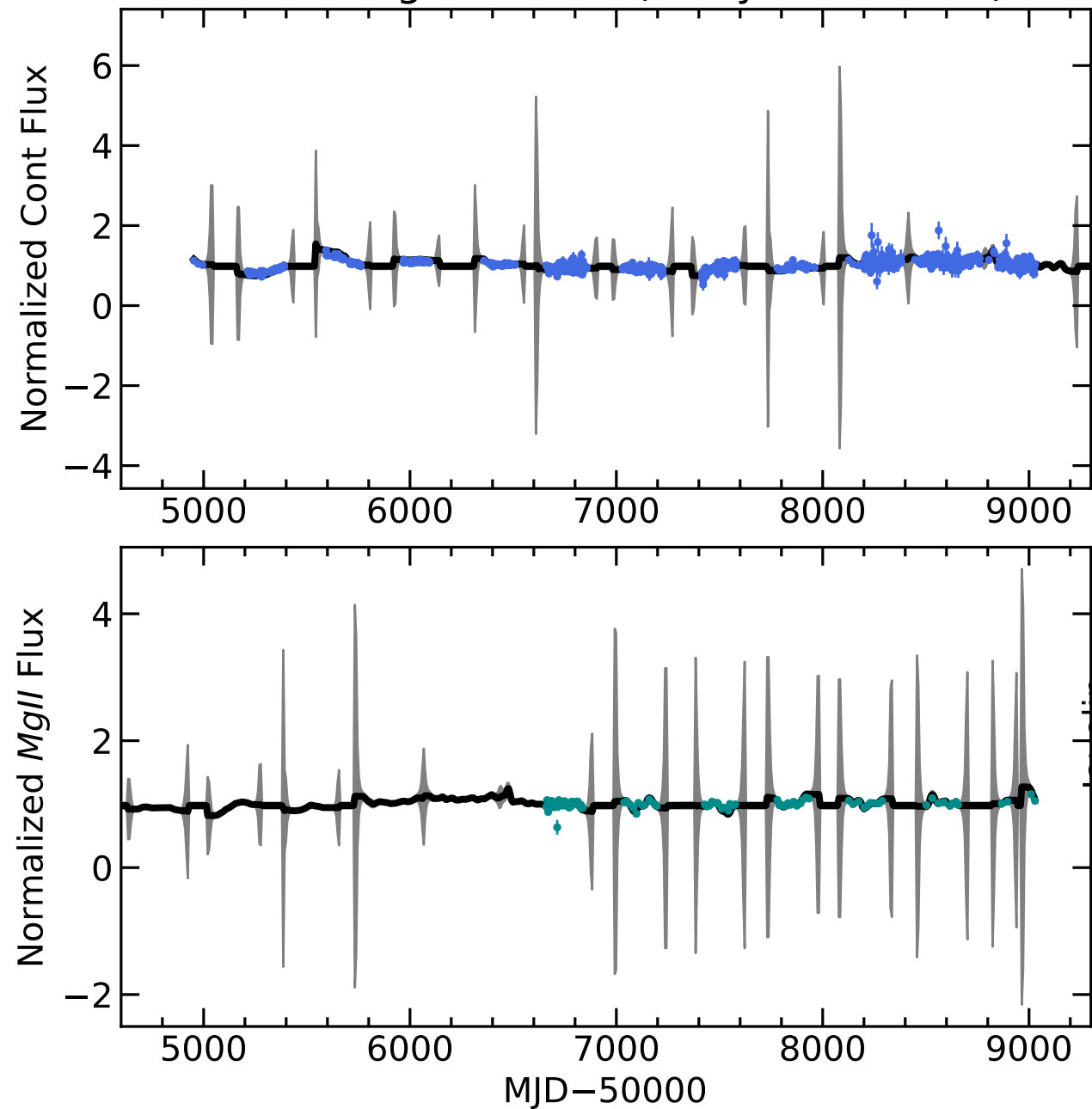
RM124 Light Curves (w/ PyROA model)
