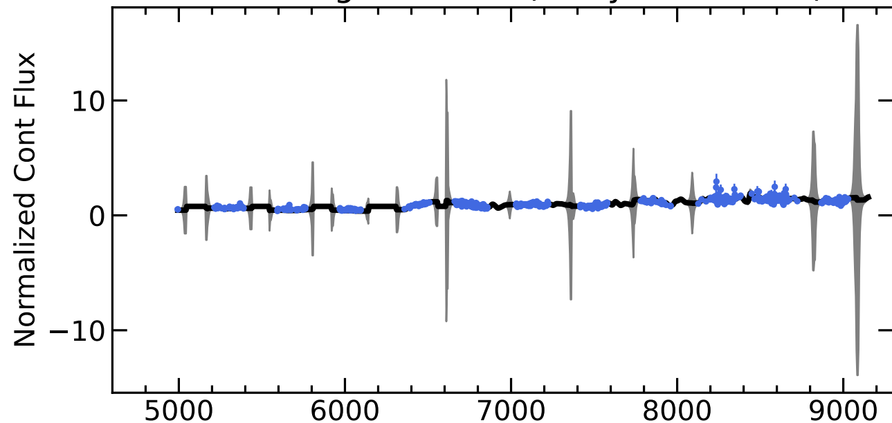
RM125 Light Curves (w/ PyROA model)
