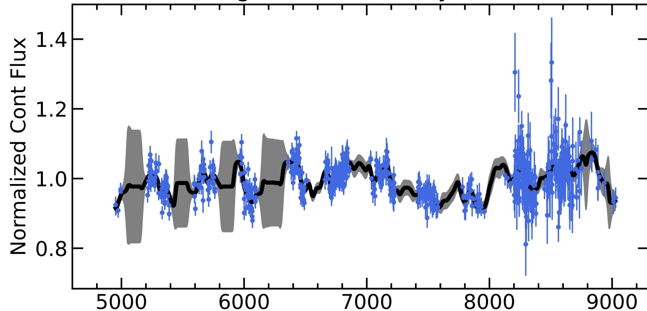
RM126 Light Curves (w/ PyROA model)
