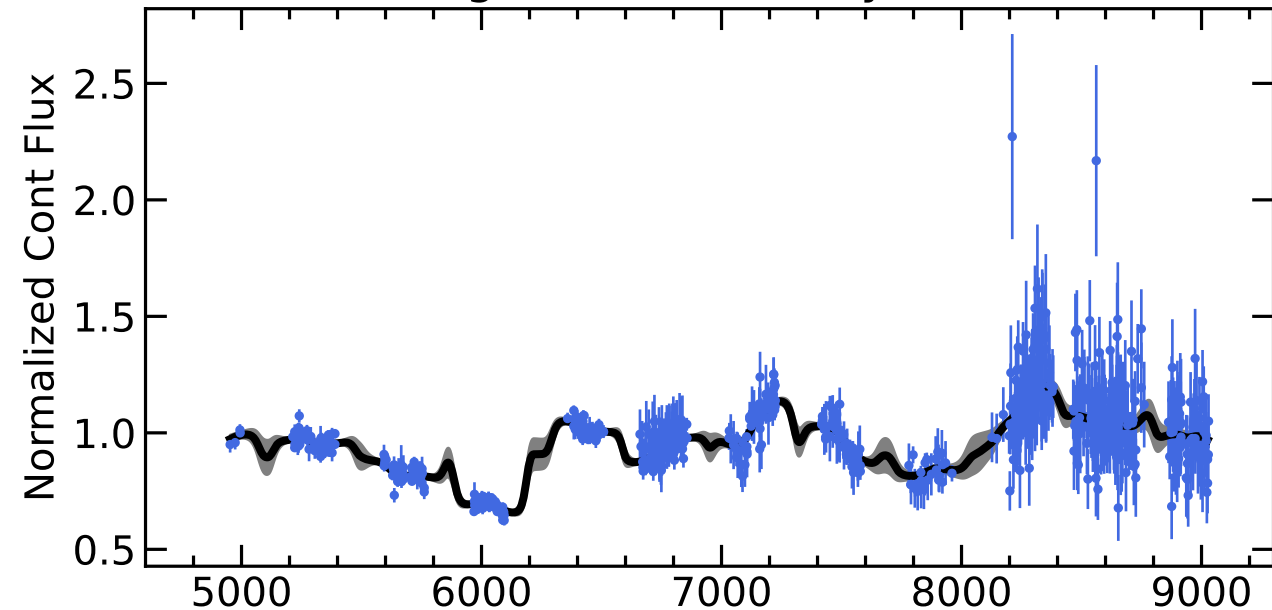
RM128 Light Curves (w/ PyROA model)
