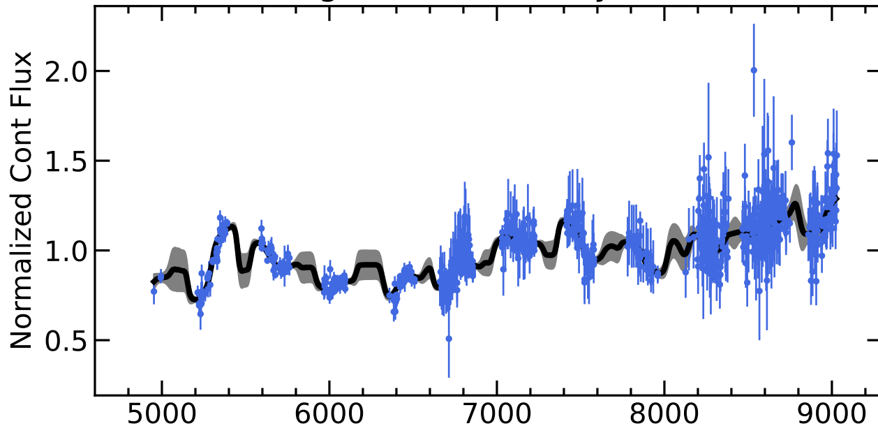
RM129 Light Curves (w/ PyROA model)
