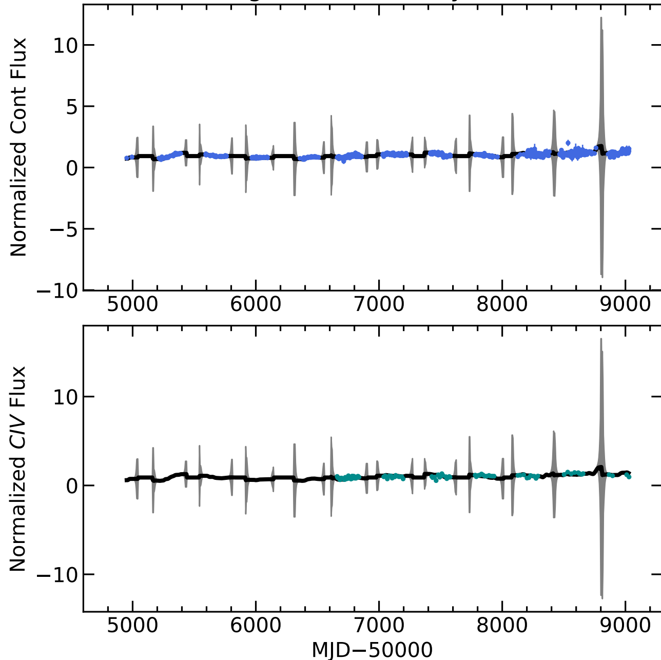
RM129 Light Curves (w/ PyROA model)
