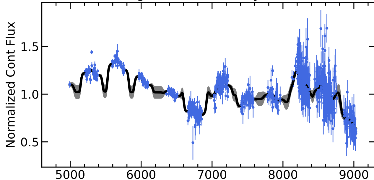
RM130 Light Curves (w/ PyROA model)
