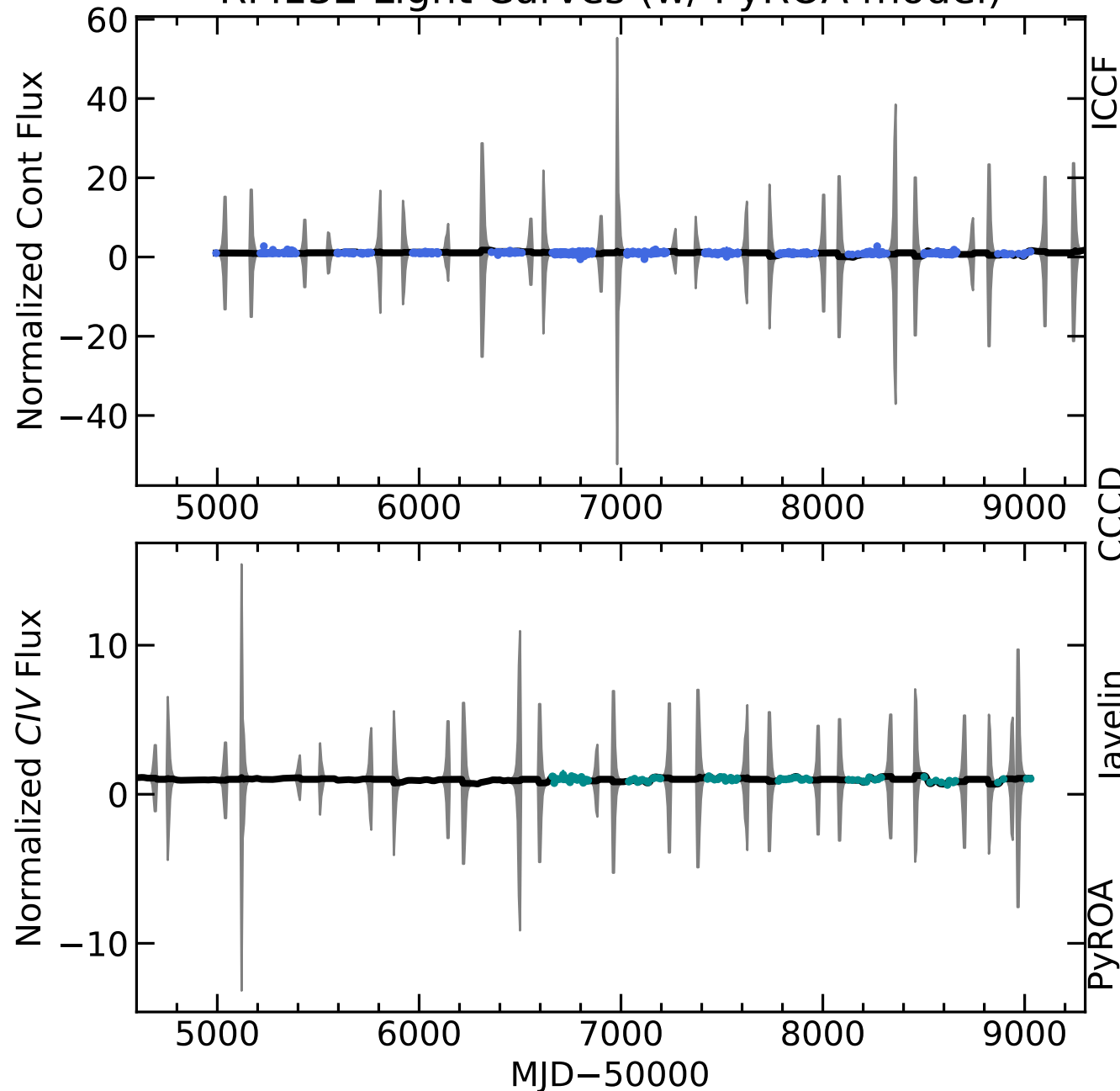
RM132 Light Curves (w/ PyROA model)
