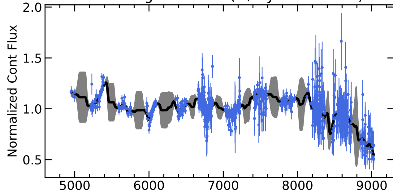
RM133 Light Curves (w/ PyROA model)
