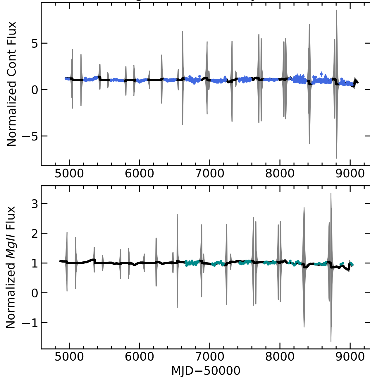
RM133 Light Curves (w/ PyROA model)
