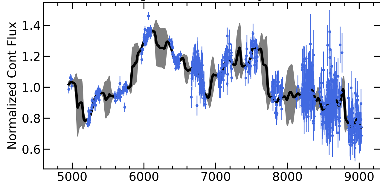
RM135 Light Curves (w/ PyROA model)
