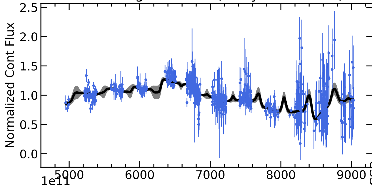
RM136 Light Curves (w/ PyROA model)
