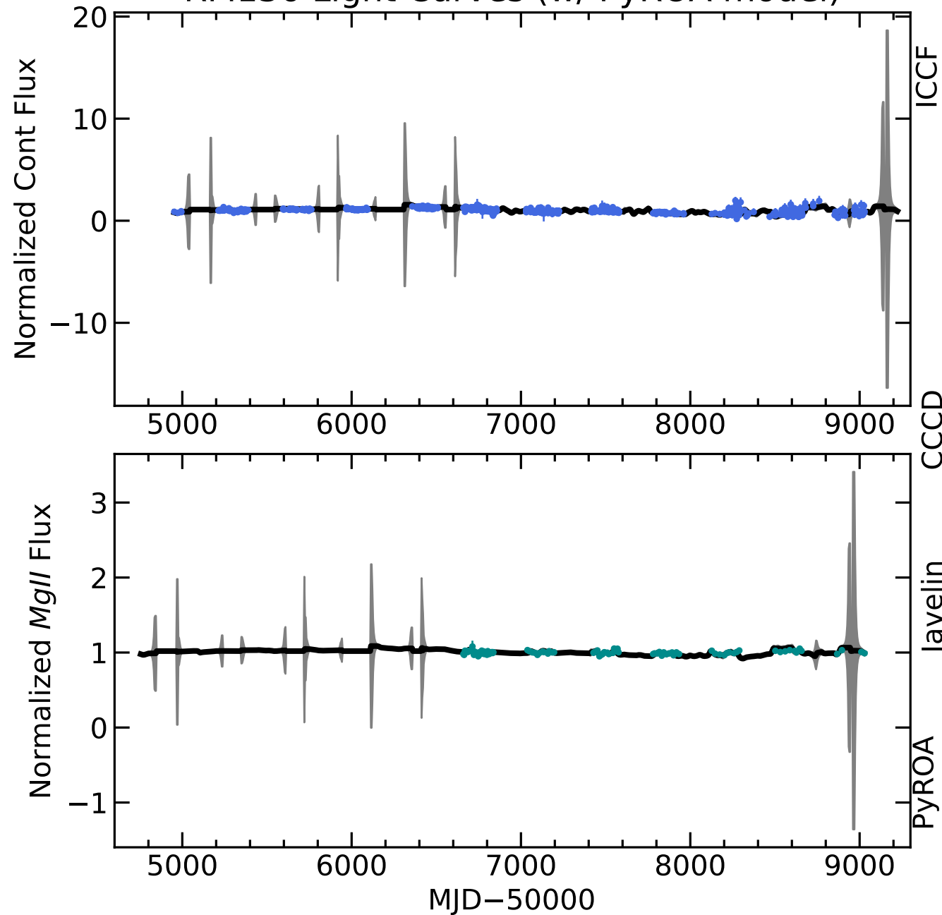
RM136 Light Curves (w/ PyROA model)
