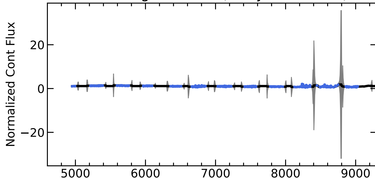
RM137 Light Curves (w/ PyROA model)
