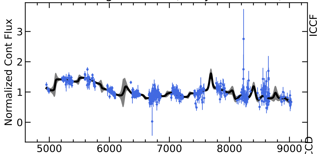
RM138 Light Curves (w/ PyROA model)
