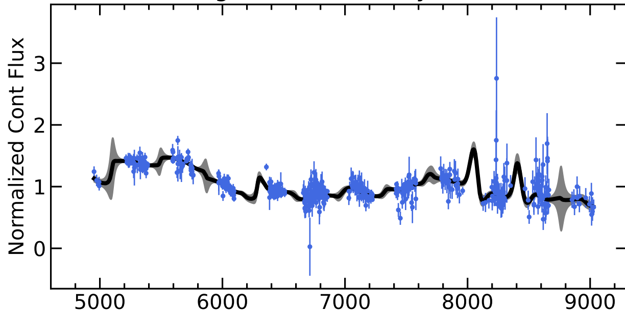
RM138 Light Curves (w/ PyROA model)
