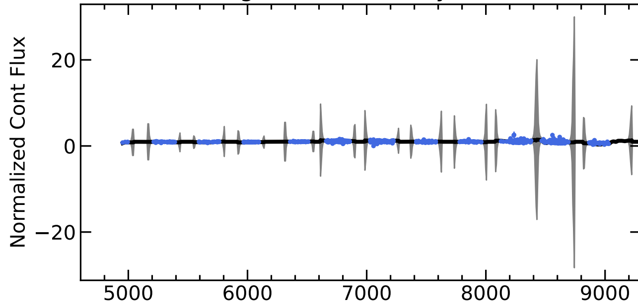
RM139 Light Curves (w/ PyROA model)
